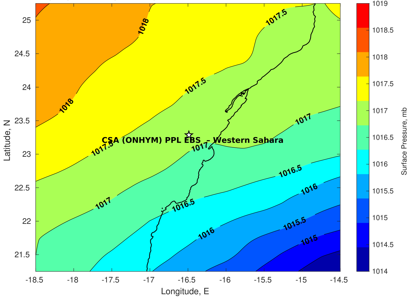
Surface Pressure (mb) for CSA (ONHYM) PPL EBS - Western Sahara at 15-Mar-2025 00:00:00
