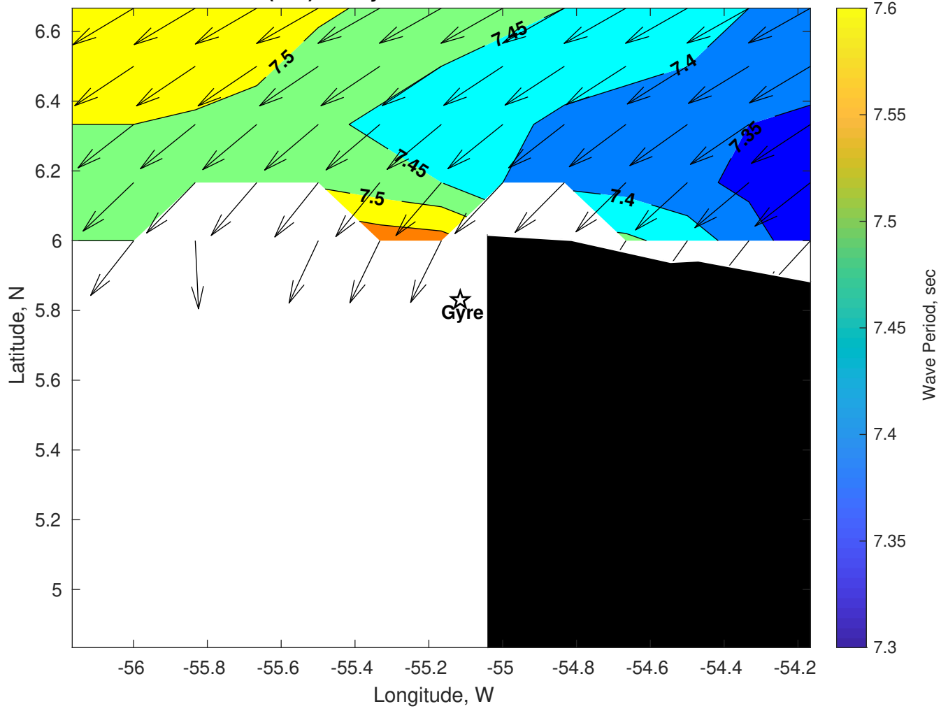
Wave Period (sec) for Gyre at 13-Mar-2025 09:00:00
