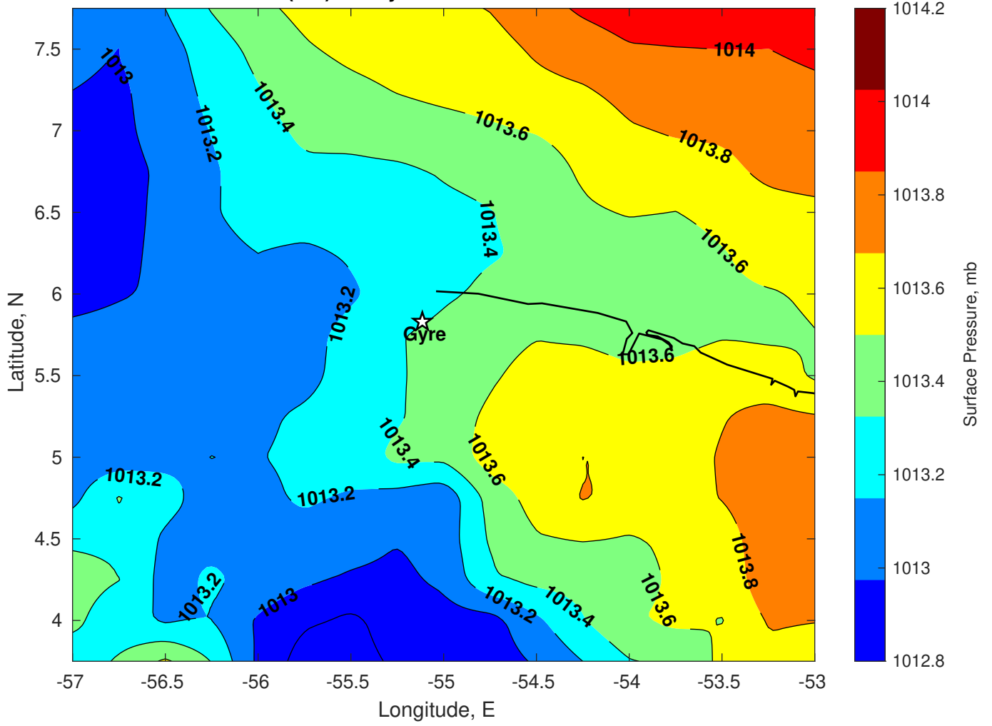
Surface Pressure (mb) for Gyre at 14-Mar-2025 00:00:00
