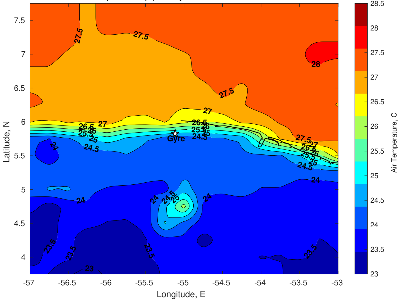
Air Temperature (C) for Gyre at 13-Mar-2025
