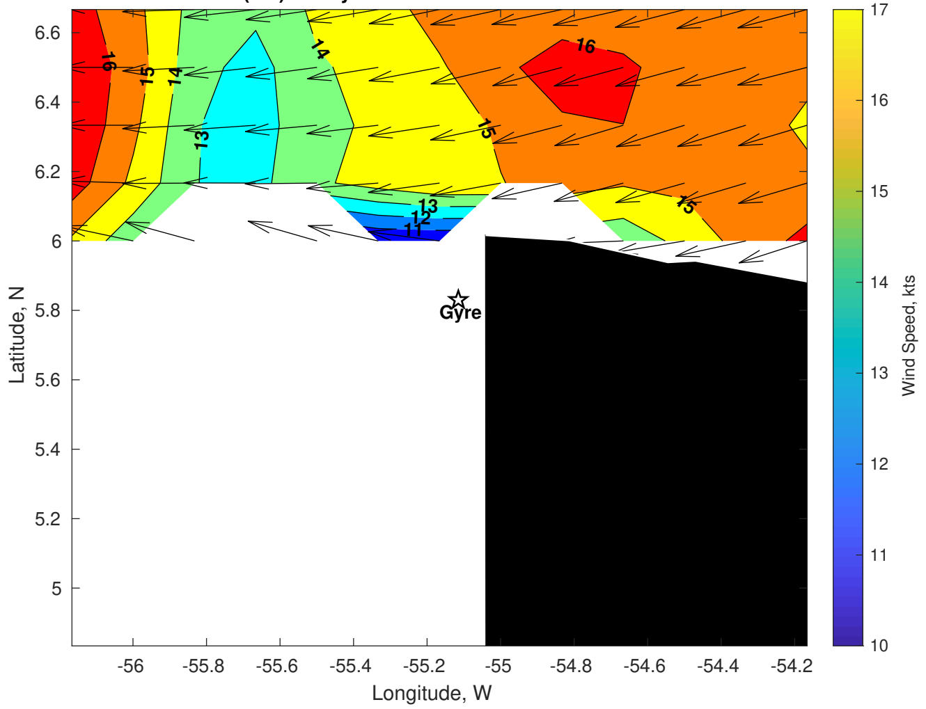
Winds (kts) for Gyre at 13-Mar-2025 09:00:00
