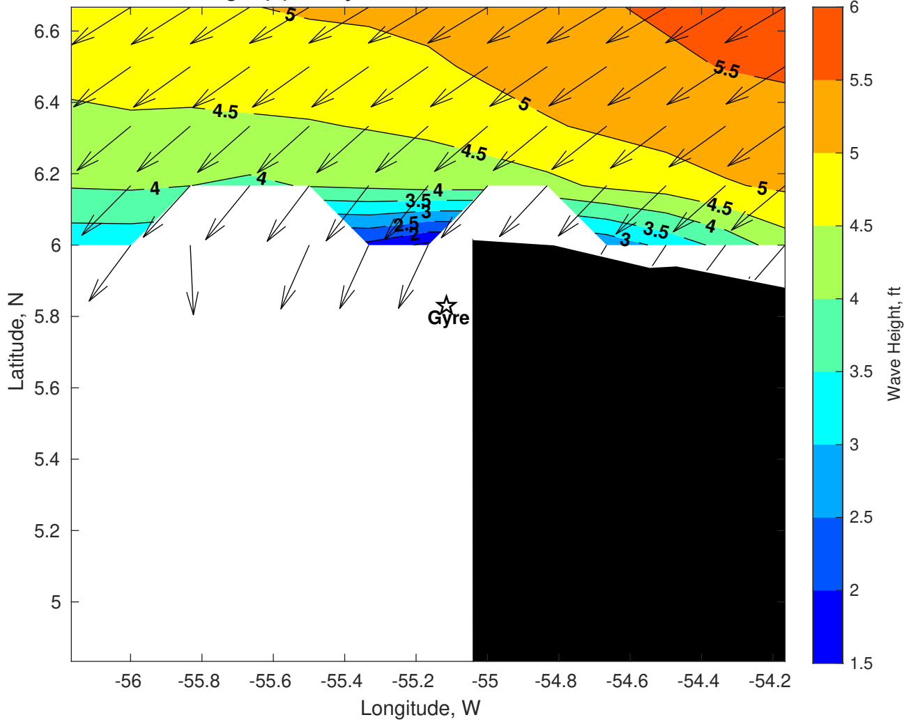
Wave Height (ft) for Gyre at 13-Mar-2025 09:00:00
