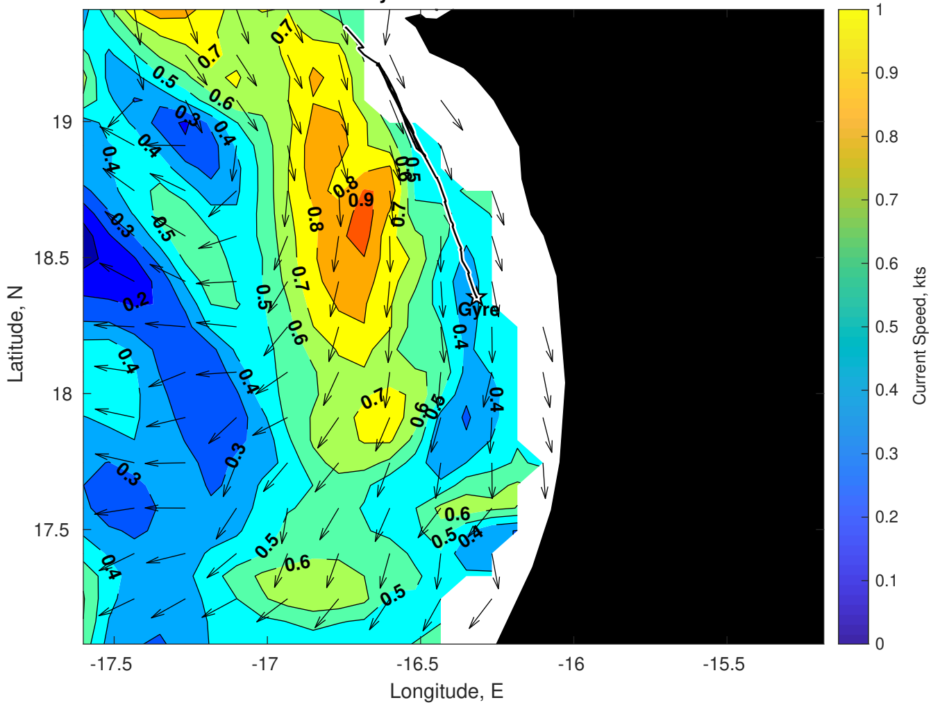
Surface Currents for Gyre at 12-Mar-2025 00:00:00
