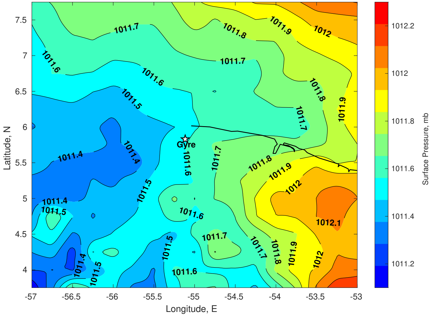
Surface Pressure (mb) for Gyre at 15-Mar-2025 00:00:00
