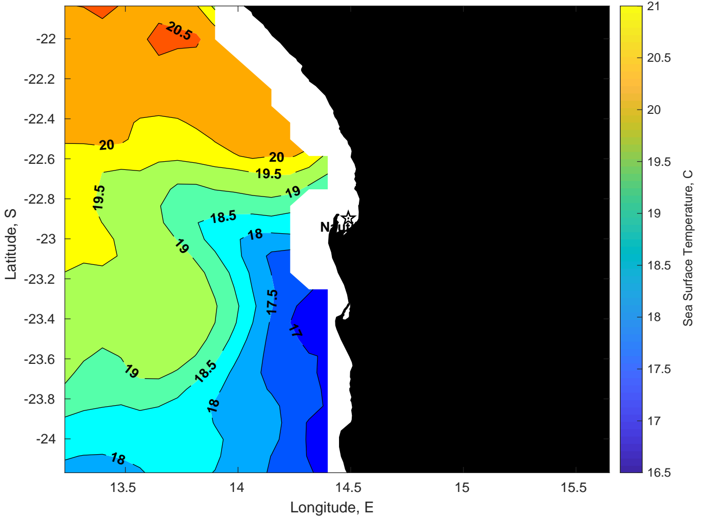
SST for Nautilus at 12-Mar-2025 00:00:00
