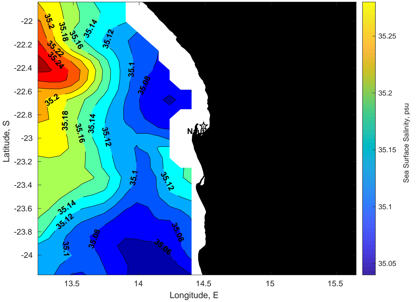
Surface Salinity for Nautilus at 12-Mar-2025 00:00:00
