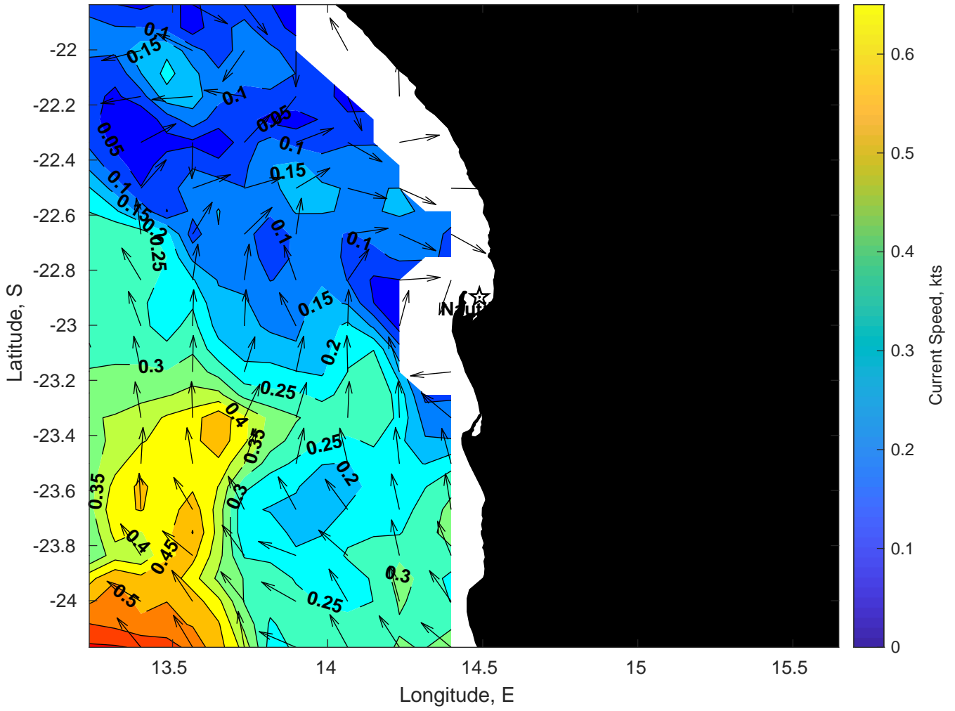
Surface Currents for Nautilus at 12-Mar-2025 00:00:00
