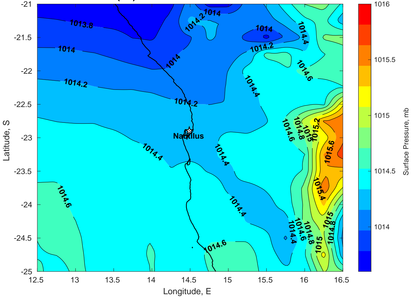
Surface Pressure (mb) for Nautilus at 15-Mar-2025 00:00:00
