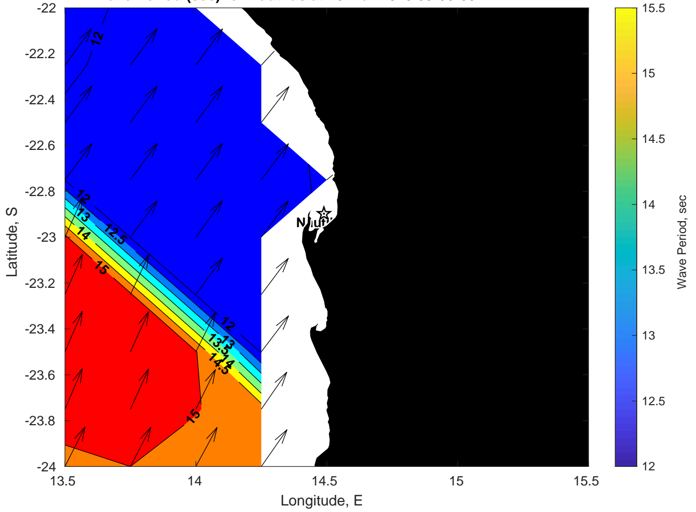
Wave Period (sec) for Nautilus at 13-Mar-2025 09:00:00
