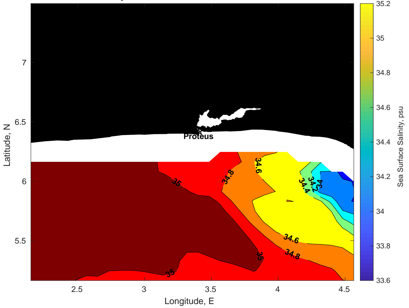
Surface Salinity for Proteus at 12-Mar-2025 00:00:00
