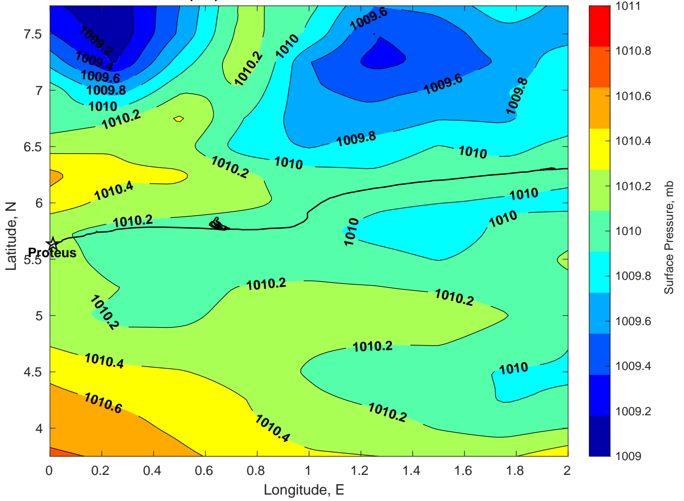
Surface Pressure (mb) for Proteus at 15-Mar-2025 00:00:00
