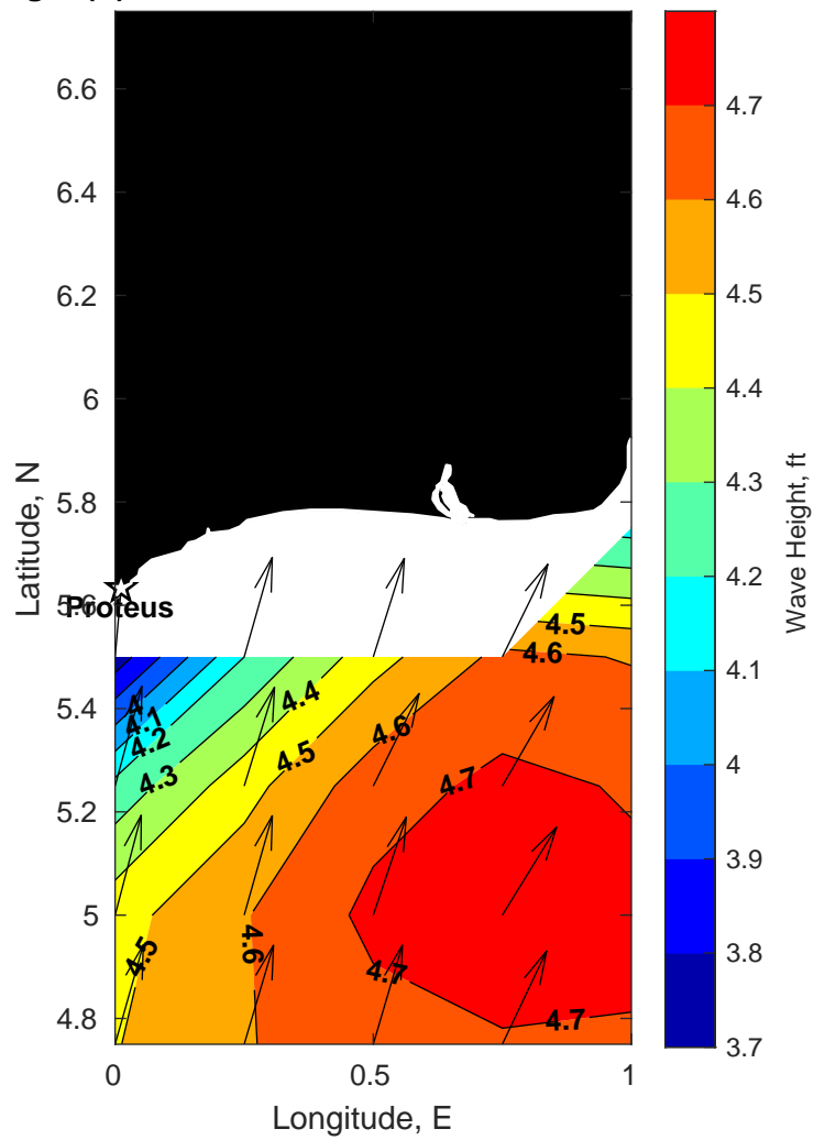
Wave Height (ft) for Proteus at 13-Mar-2025 09:00:00
