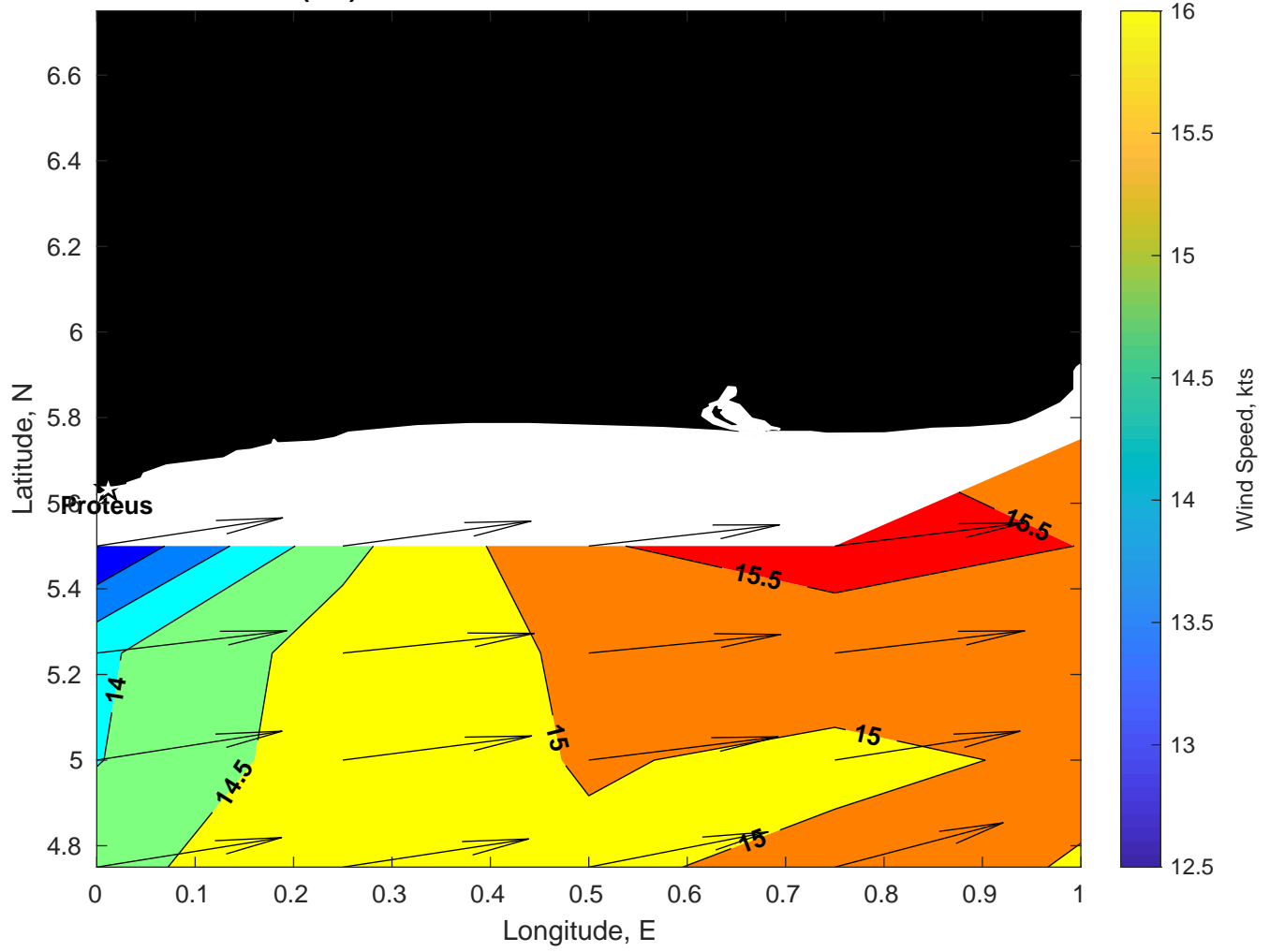
Winds (kts) for Proteus at 13-Mar-2025 09:00:00
