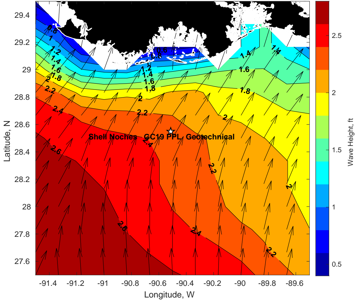
Wave Height (ft) for Shell Noches GC19 PPL Geotechnical at 13-Mar-2025 09:00:00
