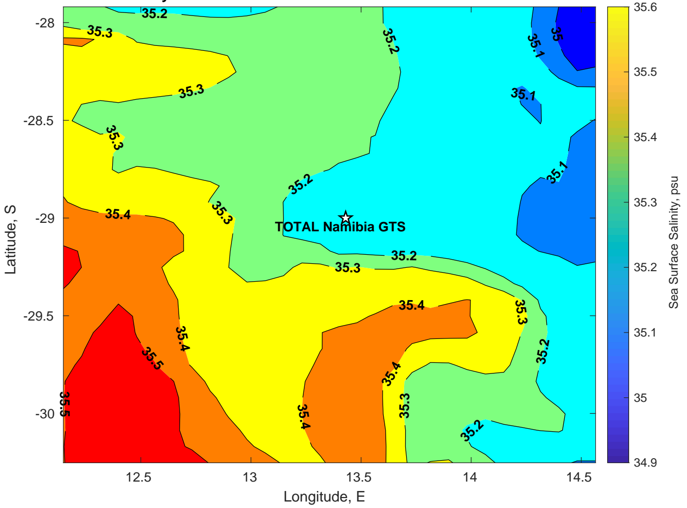
Surface Salinity for TOTAL Namibia GTS at 12-Mar-2025 00:00:00
