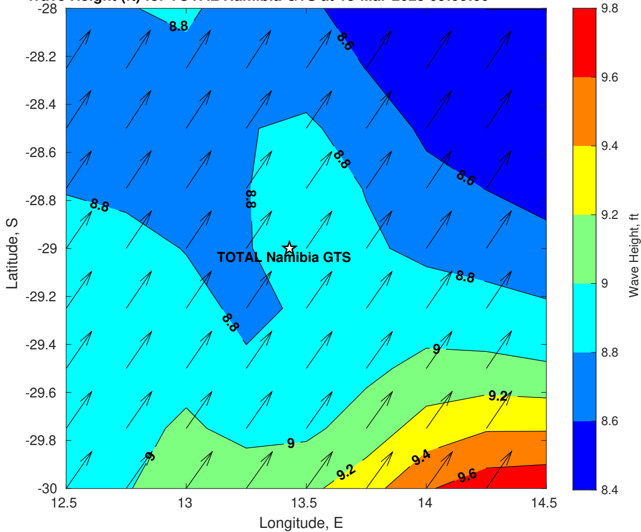
Wave Height (ft) for TOTAL Namibia GTS at 13-Mar-2025 09:00:00
