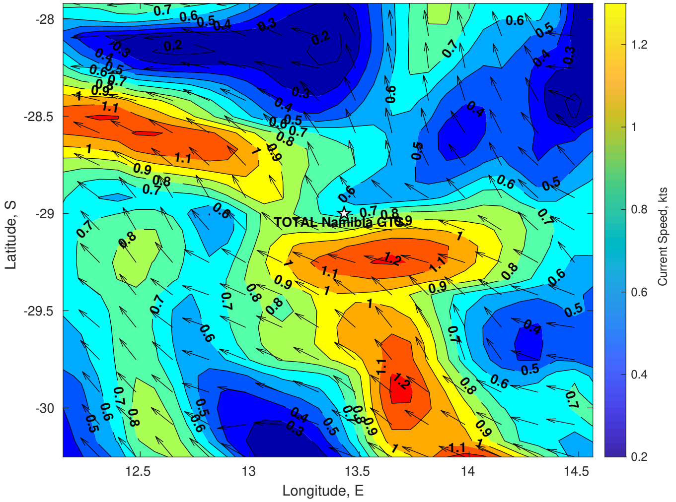
Surface Currents for TOTAL Namibia GTS at 12-Mar-2025 00:00:00
