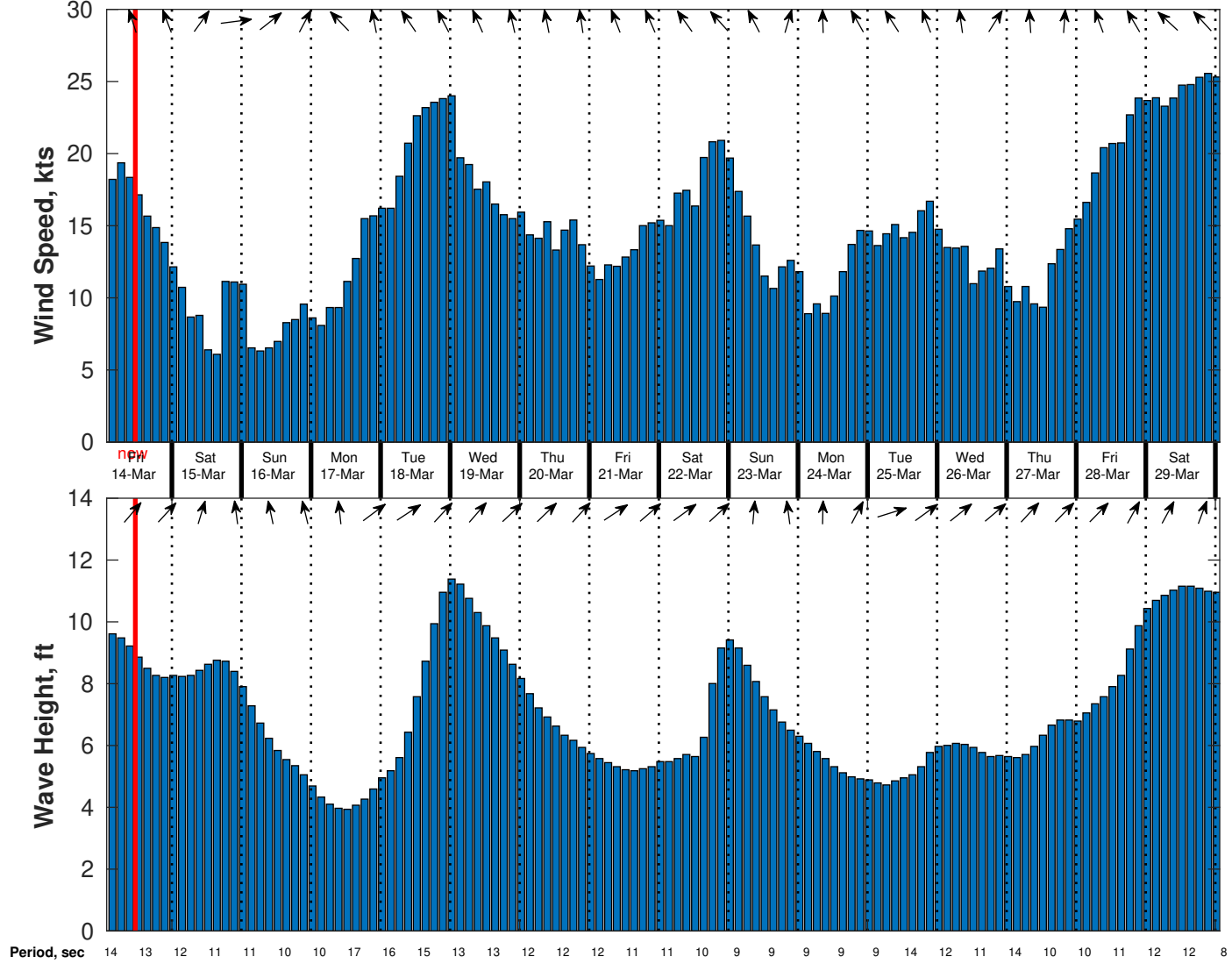
Wind & Wave Forecast for TOTAL Namibia GTS from 13-Mar-2025 02:00:00 to 29-Mar-2025 02:00:00
