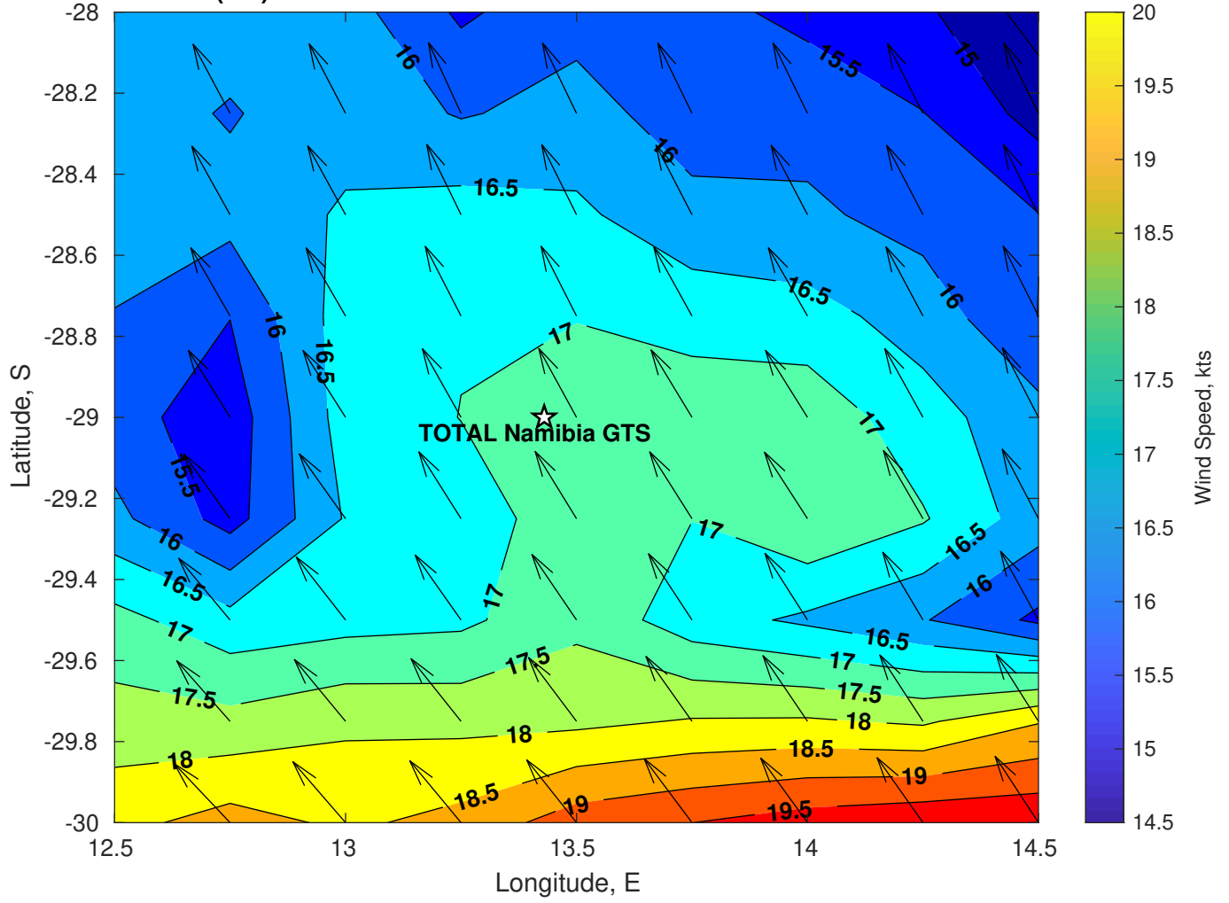
Winds (kts) for TOTAL Namibia GTS at 13-Mar-2025 09:00:00
