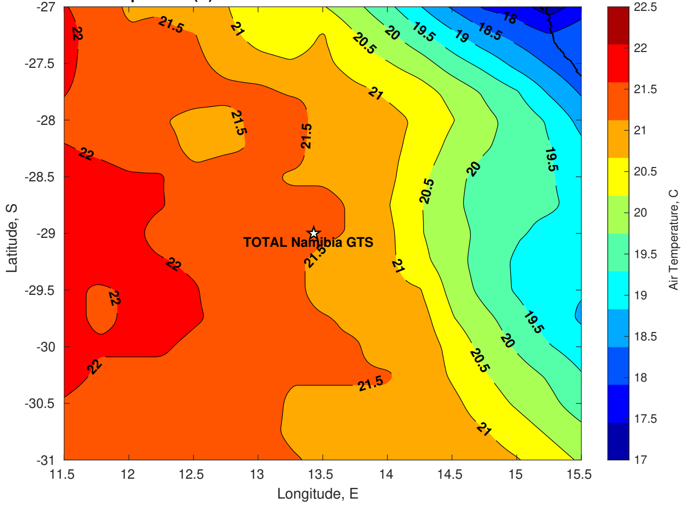
Air Temperature (C) for TOTAL Namibia GTS at 13-Mar-2025
