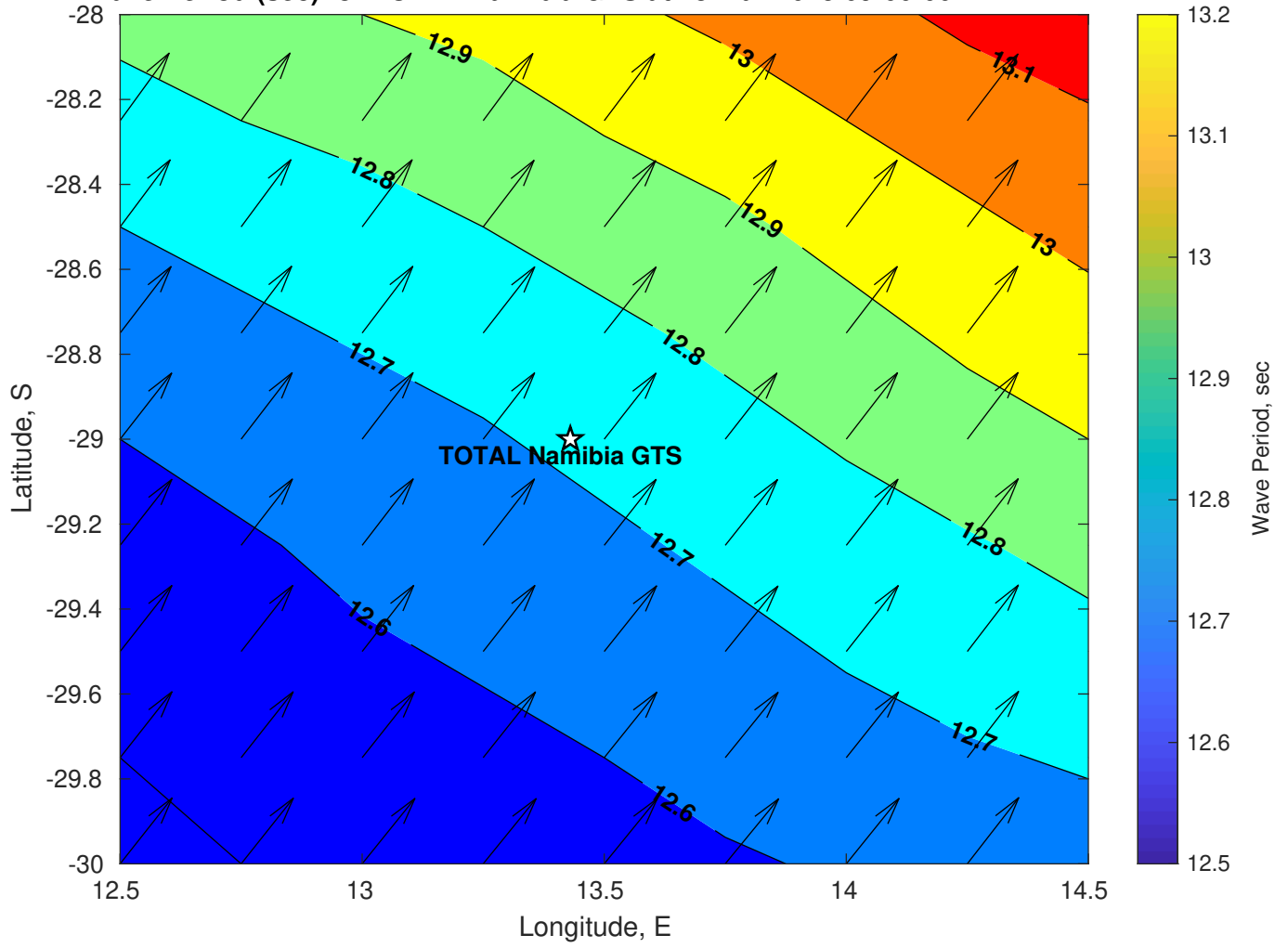
Wave Period (sec) for TOTAL Namibia GTS at 13-Mar-2025 09:00:00
