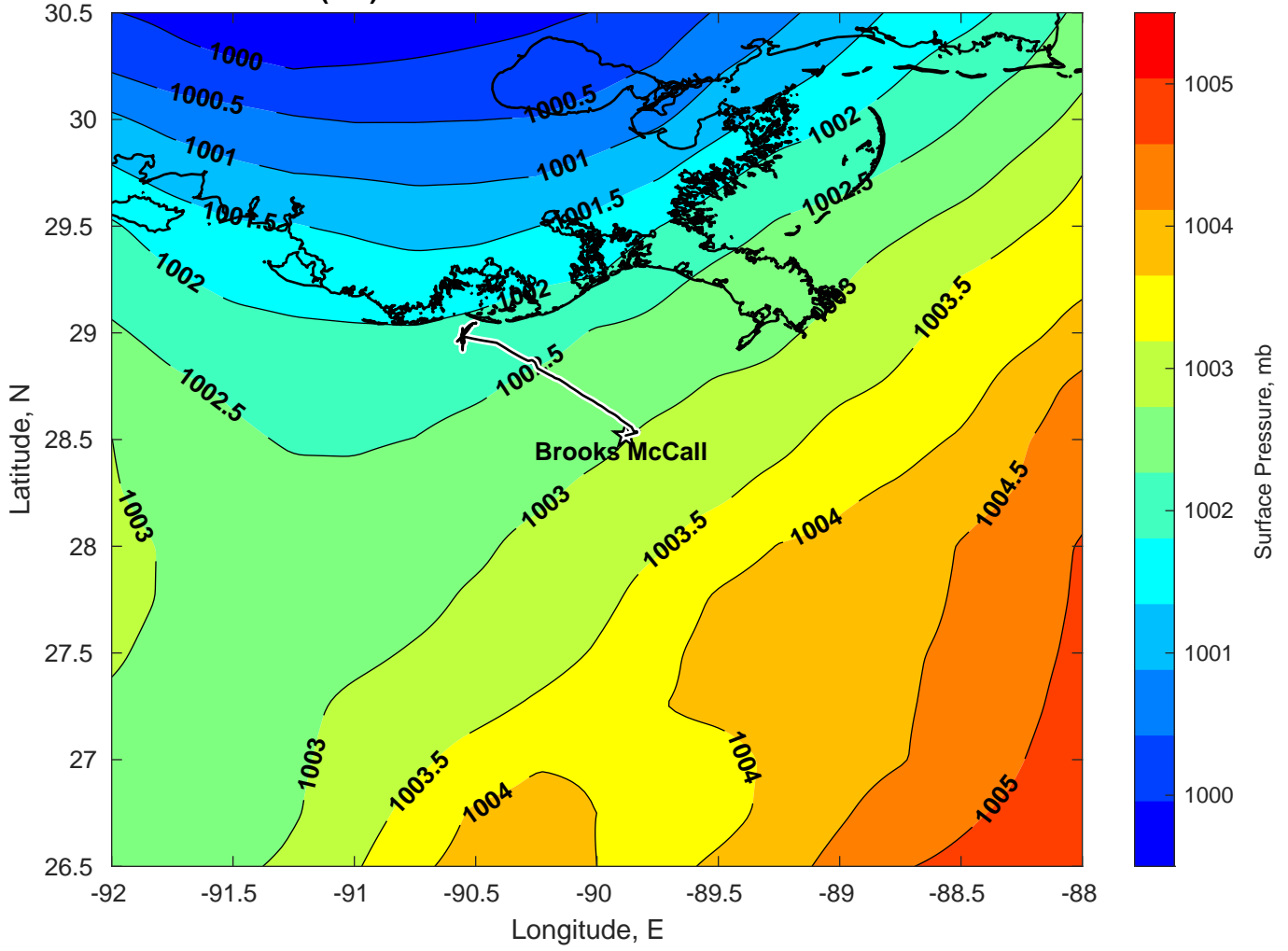
Surface Pressure (mb) for Brooks McCall at 16-Mar-2025 00:00:00
