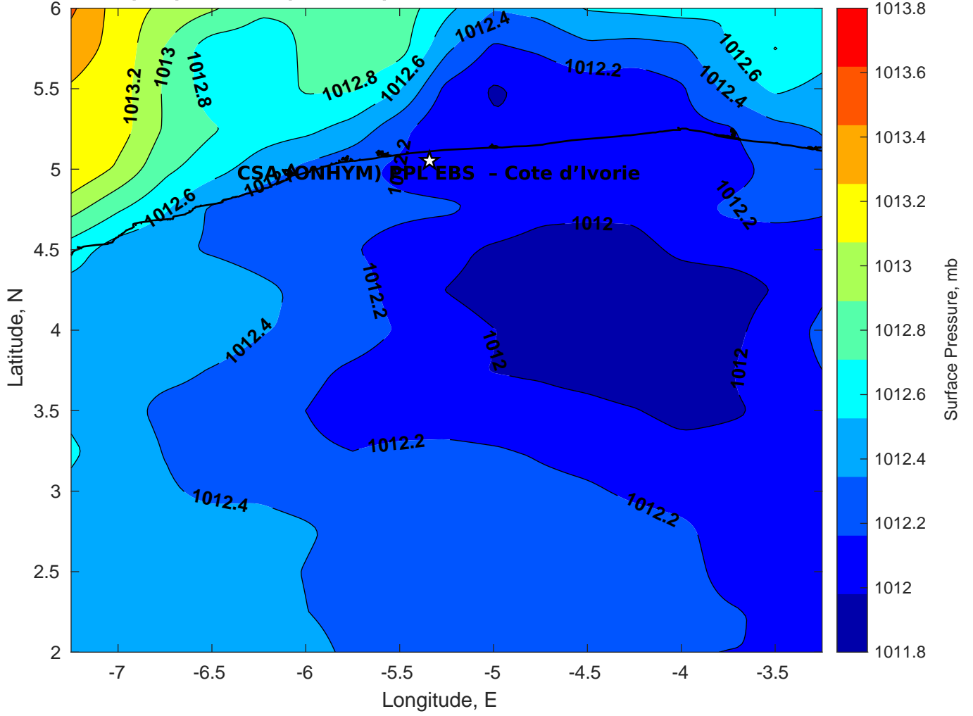
Surface Pressure (mb) for CSA (ONHYM) PPL EBS - Cote d'Ivoire at 16-Mar-2025 00:00:00
