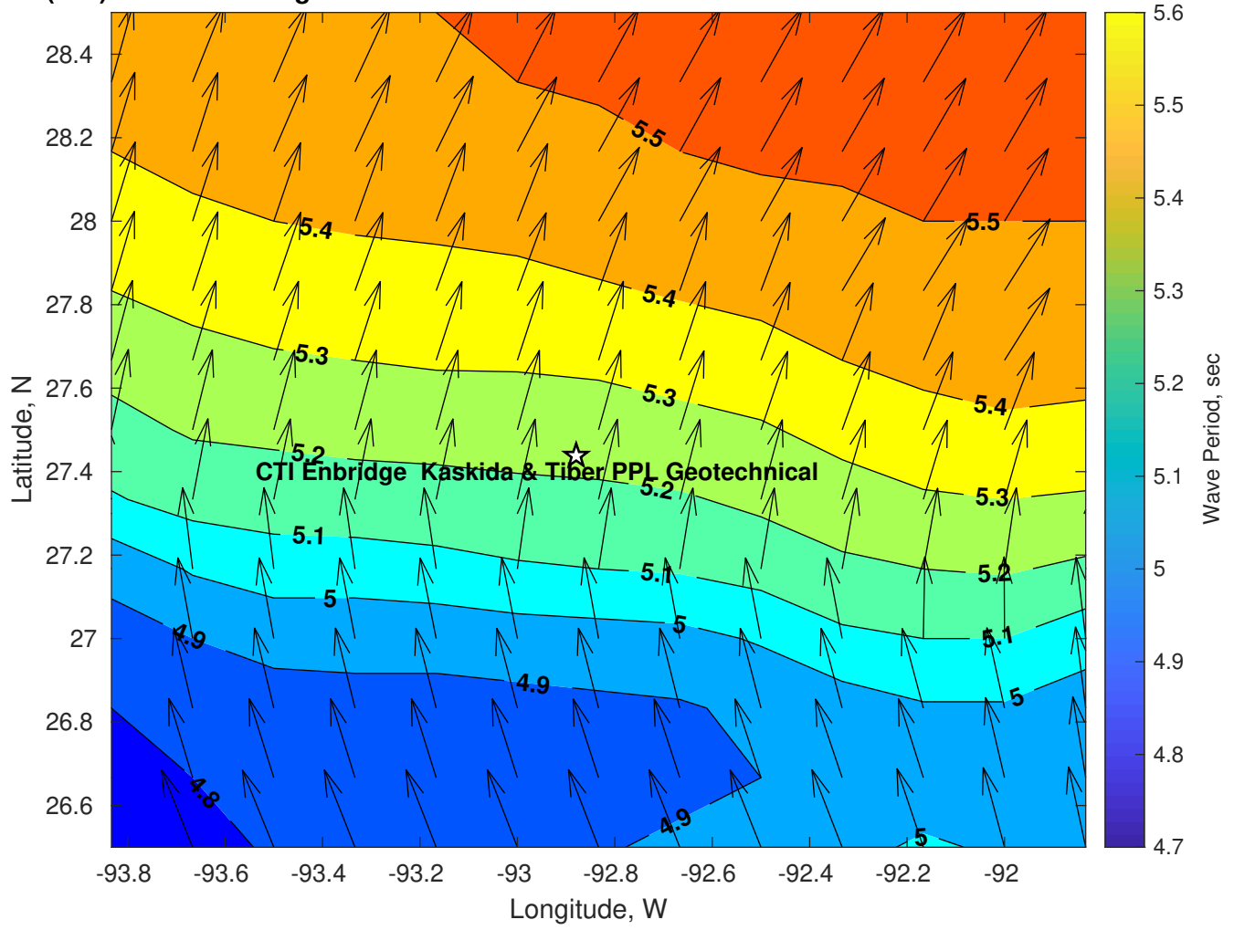
Wave Period (sec) for CTI Enbridge Kaskida & Tiber PPL Geotechnical at 14-Mar-2025 09:00:00
