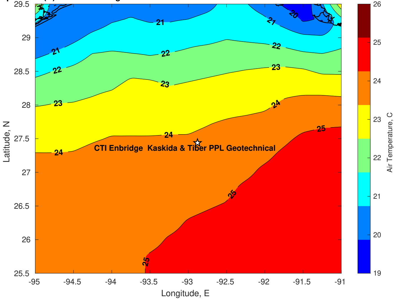
Air Temperature (C) for CTI Enbridge Kaskida & Tiber PPL Geotechnical at 14-Mar-2025
