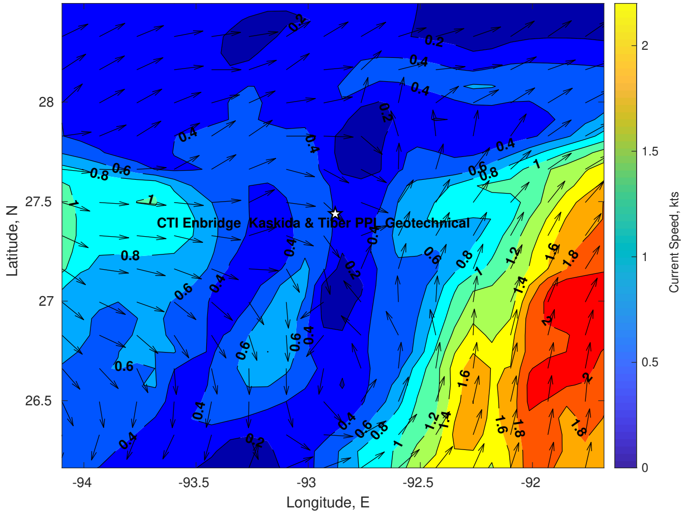
Surface Currents for CTI Enbridge Kaskida & Tiber PPL Geotechnical at 13-Mar-2025 00:00:00
