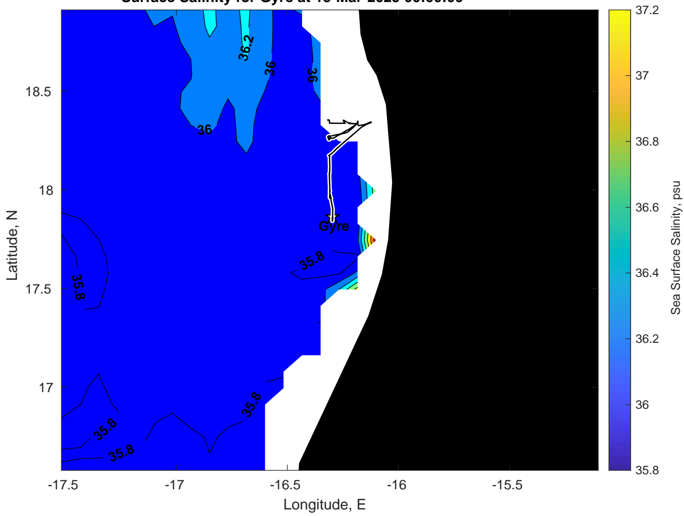
Surface Salinity for Gyre at 13-Mar-2025 00:00:00
