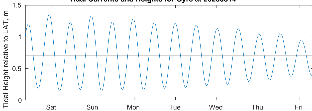
Tidal Currents and Heights for Gyre at 20250314
