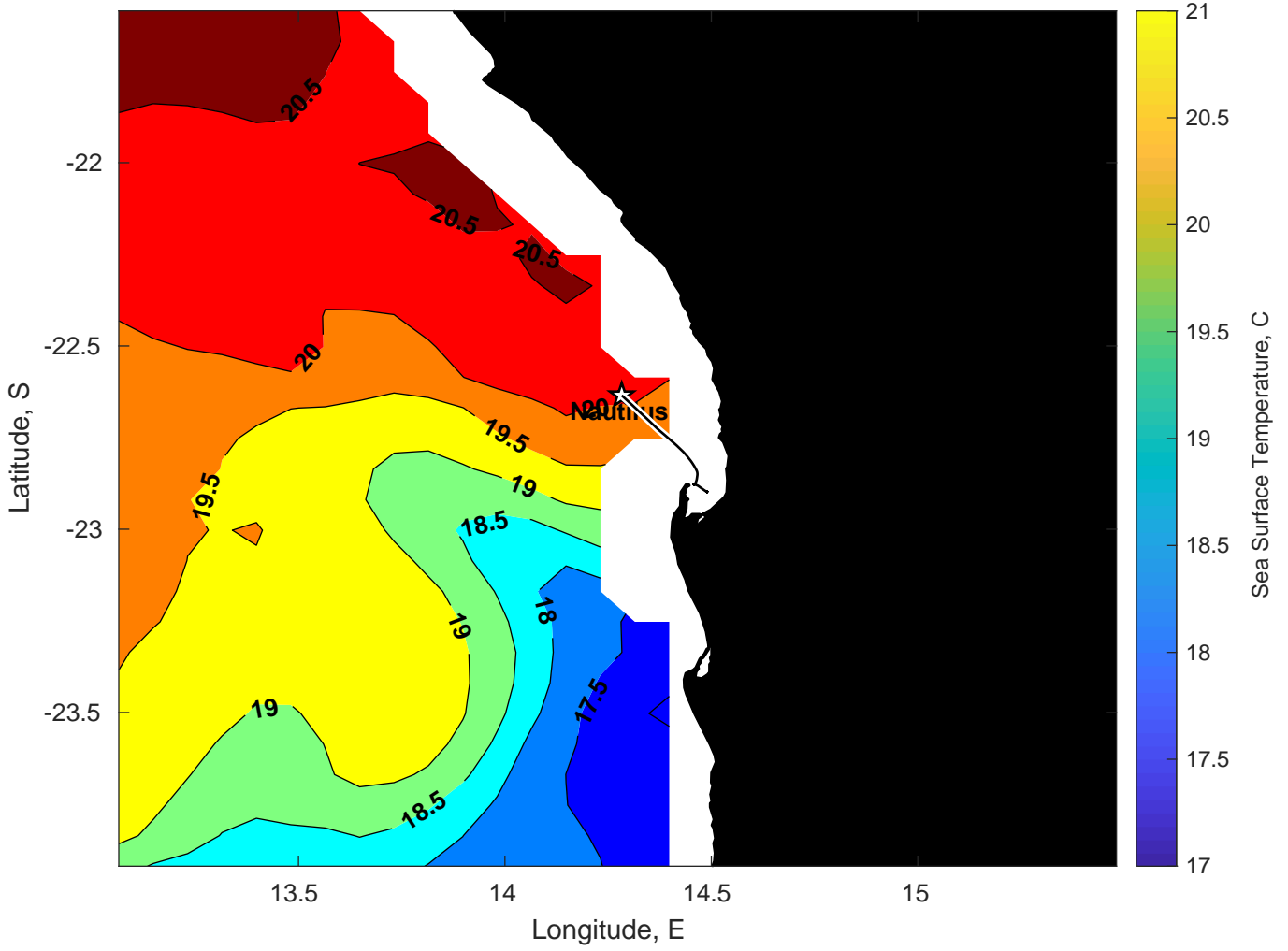
SST for Nautilus at 13-Mar-2025 00:00:00
