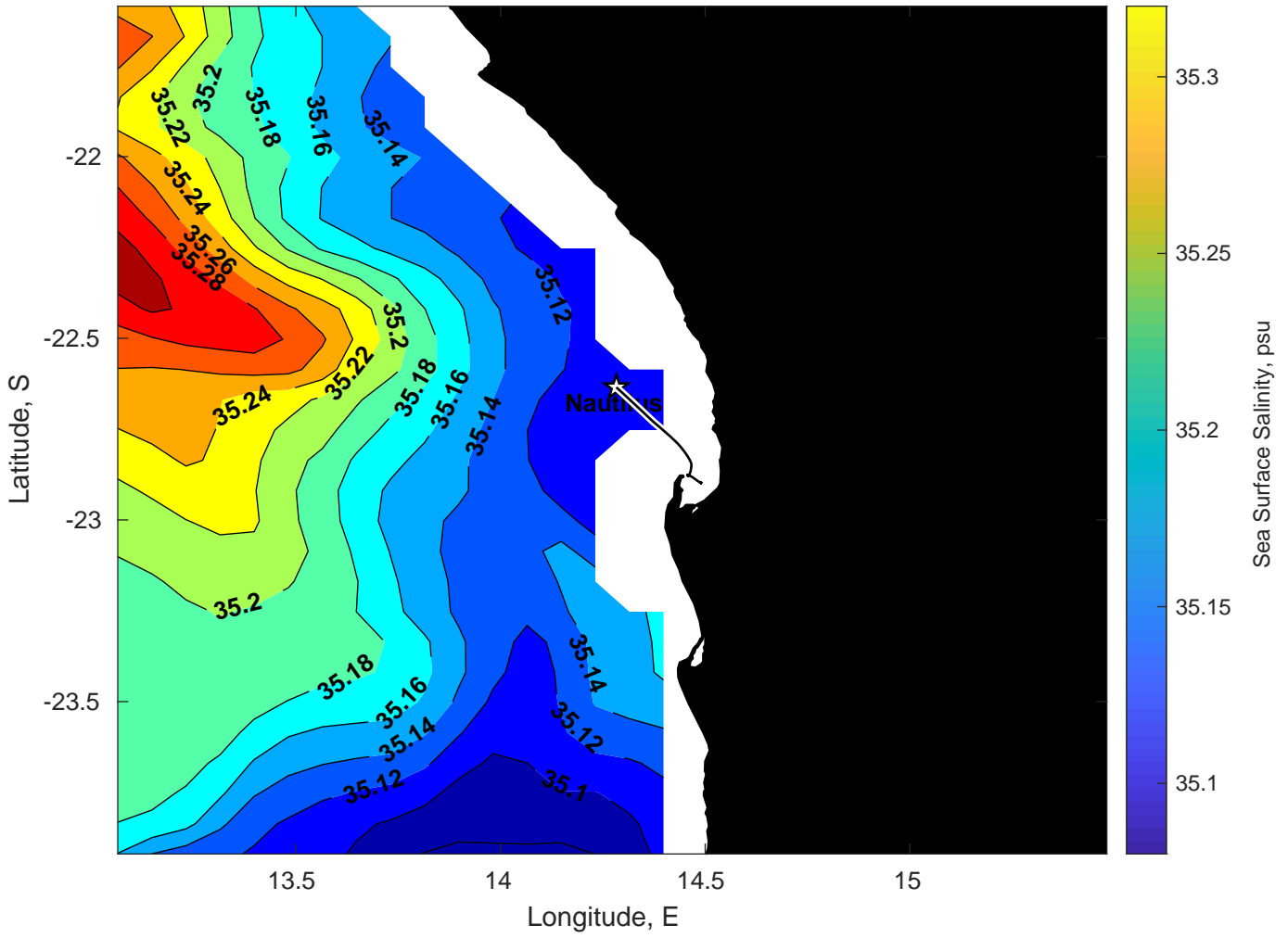
Surface Salinity for Nautilus at 13-Mar-2025 00:00:00
