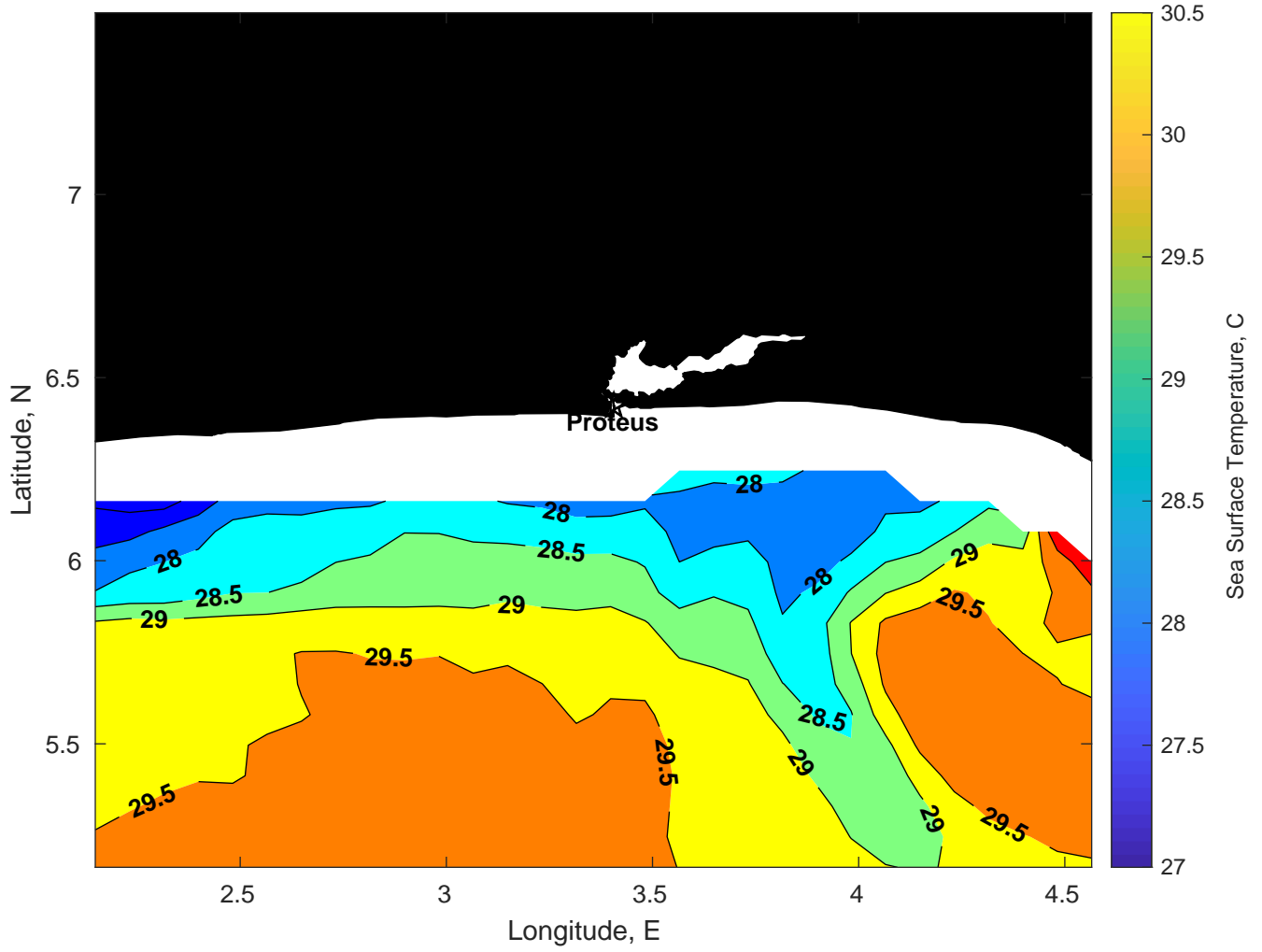
SST for Proteus at 13-Mar-2025 00:00:00
