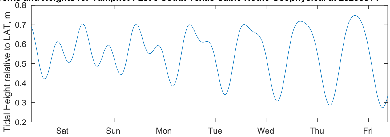
Tidal Currents and Heights for Tampnet P2378 South Texas Cable Route Geophysical at 20250314
