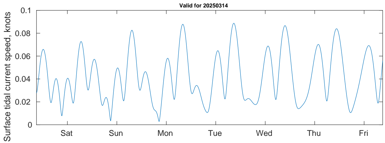
Tidal Currents and Heights for Tampnet P2378 South Texas Cable Route Geophysical at 20250314
