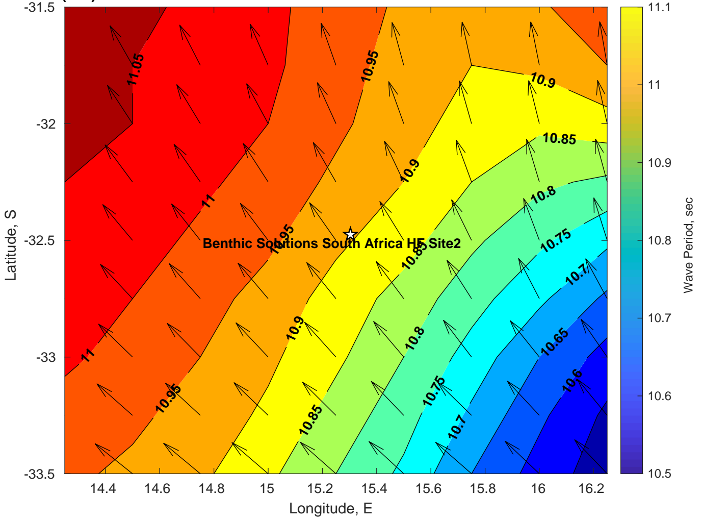
Wave Period (sec) for Benthic Solutions South Africa HF Site2 at 14-Mar-2025 09:00:00
