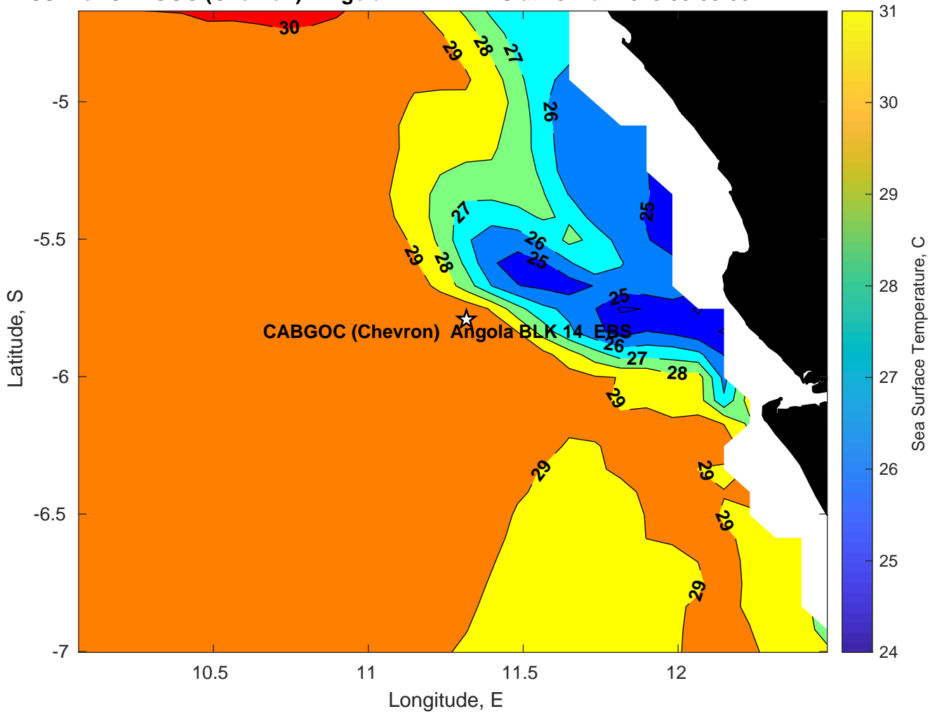
SST for CABGOC (Chevron) Angola BLK 14 EBS at 13-Mar-2025 00:00:00
