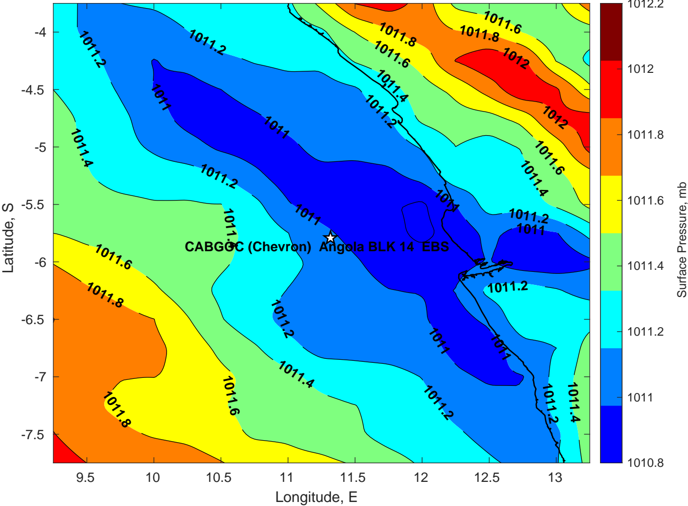
Surface Pressure (mb) for CABGOC (Chevron) Angola BLK 14 EBS at 16-Mar-2025 00:00:00
