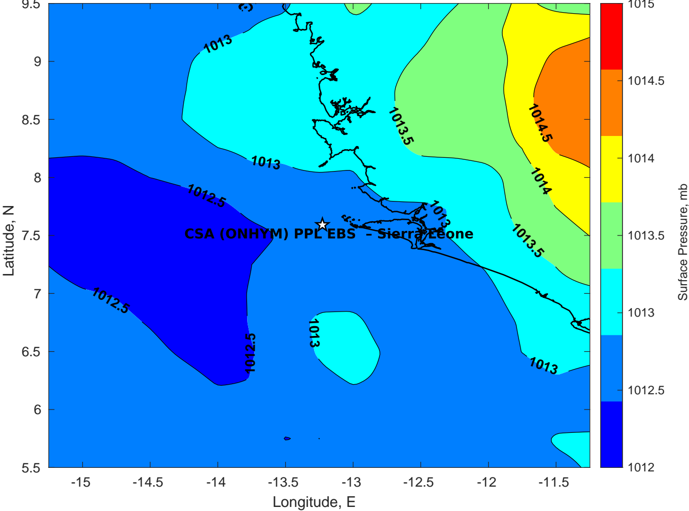
Surface Pressure (mb) for CSA (ONHYM) PPL EBS - Sierra Leone at 16-Mar-2025 00:00:00
