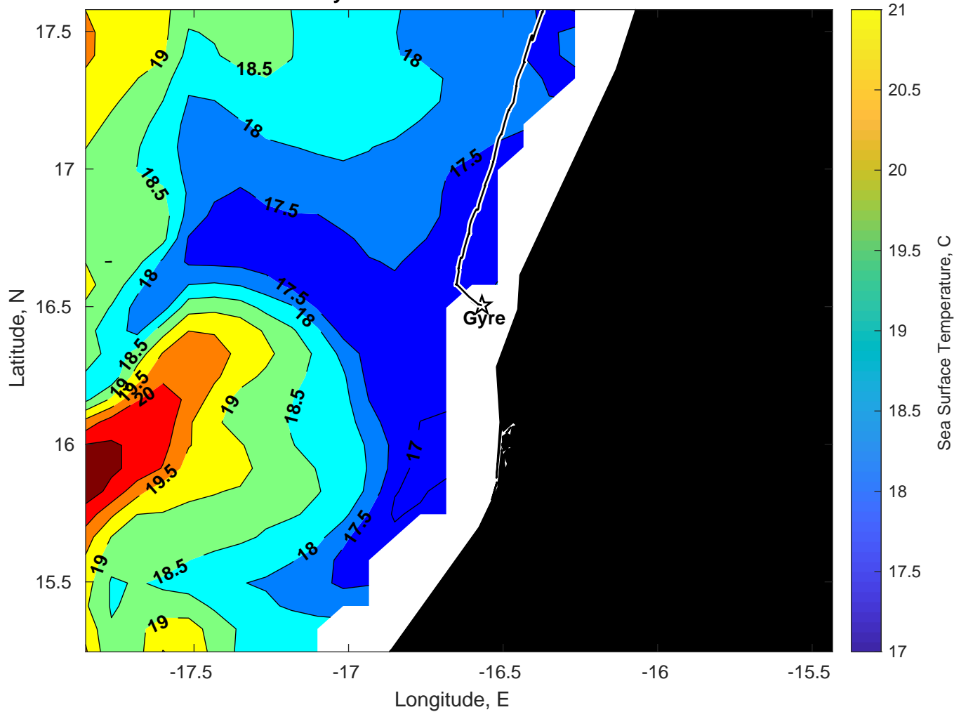
SST for Gyre at 14-Mar-2025 00:00:00
