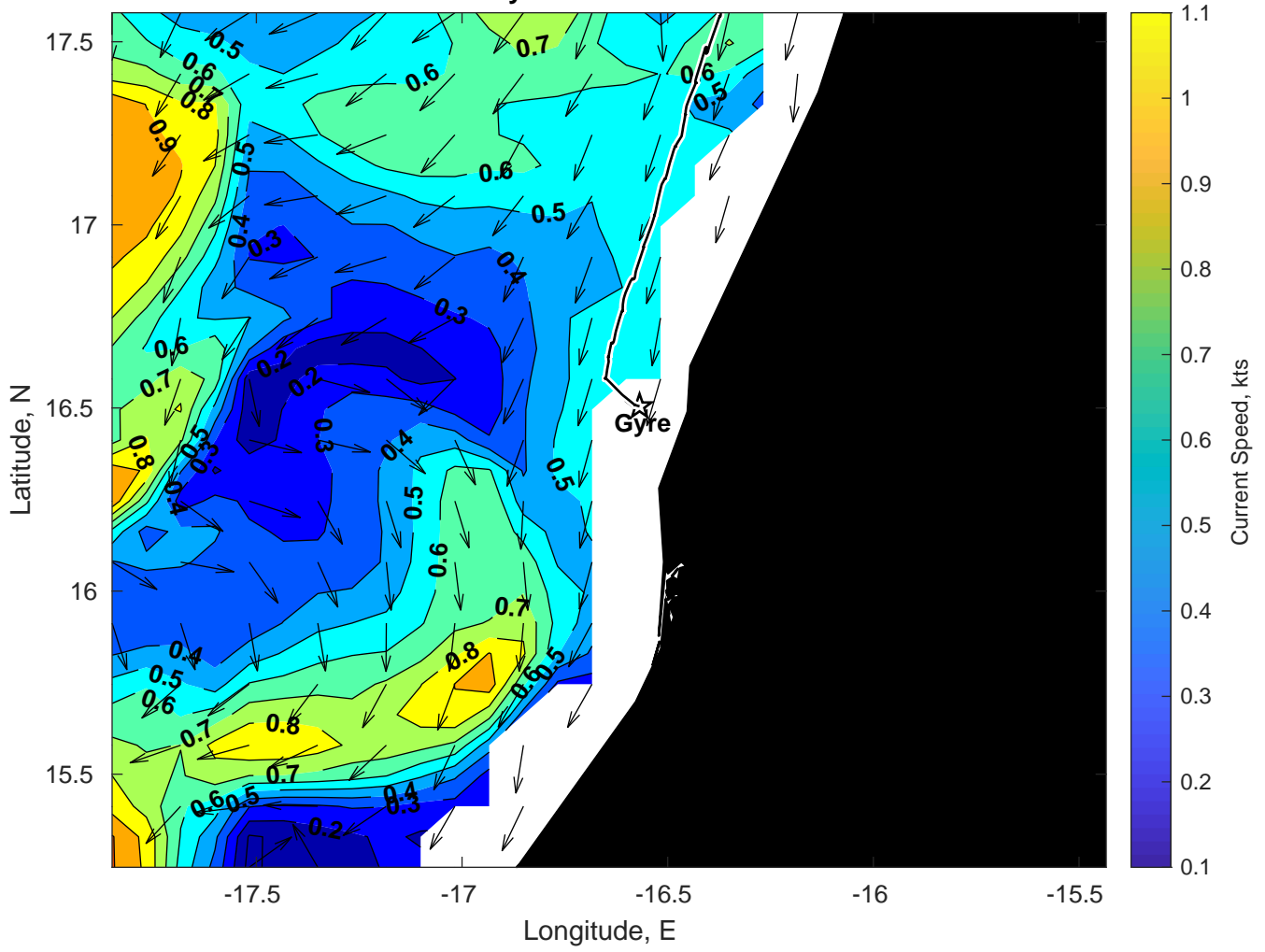
Surface Currents for Gyre at 14-Mar-2025 00:00:00
