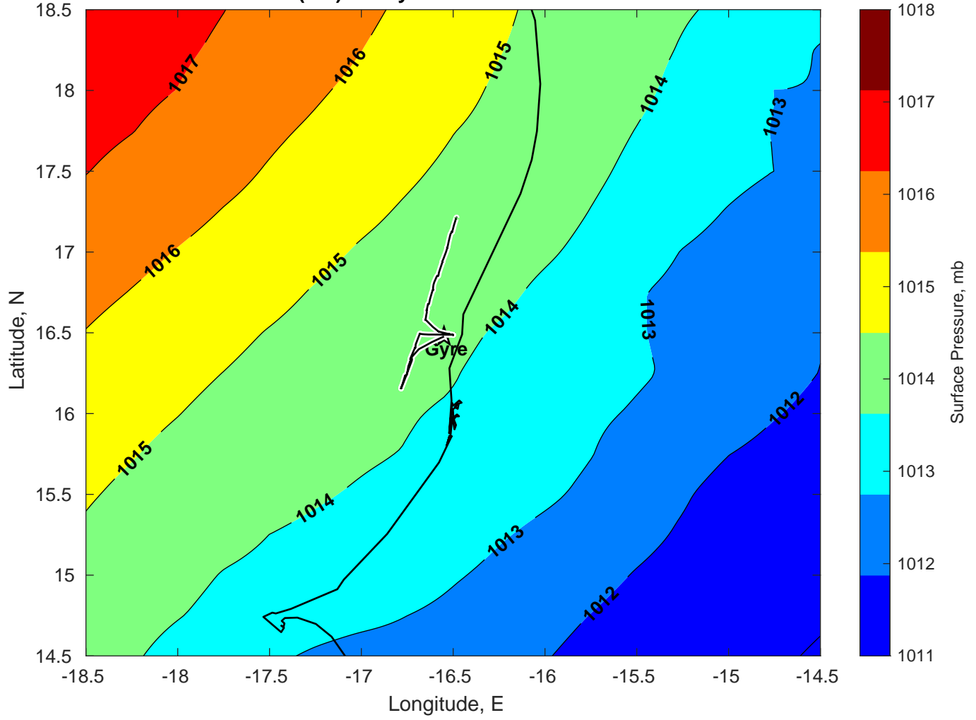
Surface Pressure (mb) for Gyre at 17-Mar-2025 00:00:00
