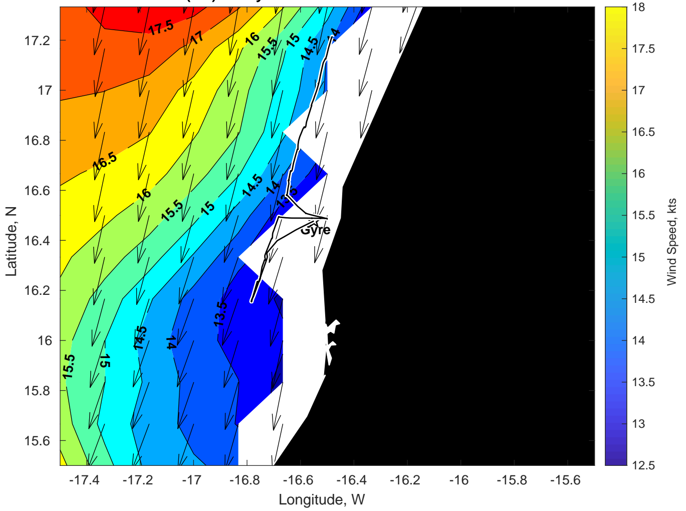
Winds (kts) for Gyre at 15-Mar-2025 09:00:00
