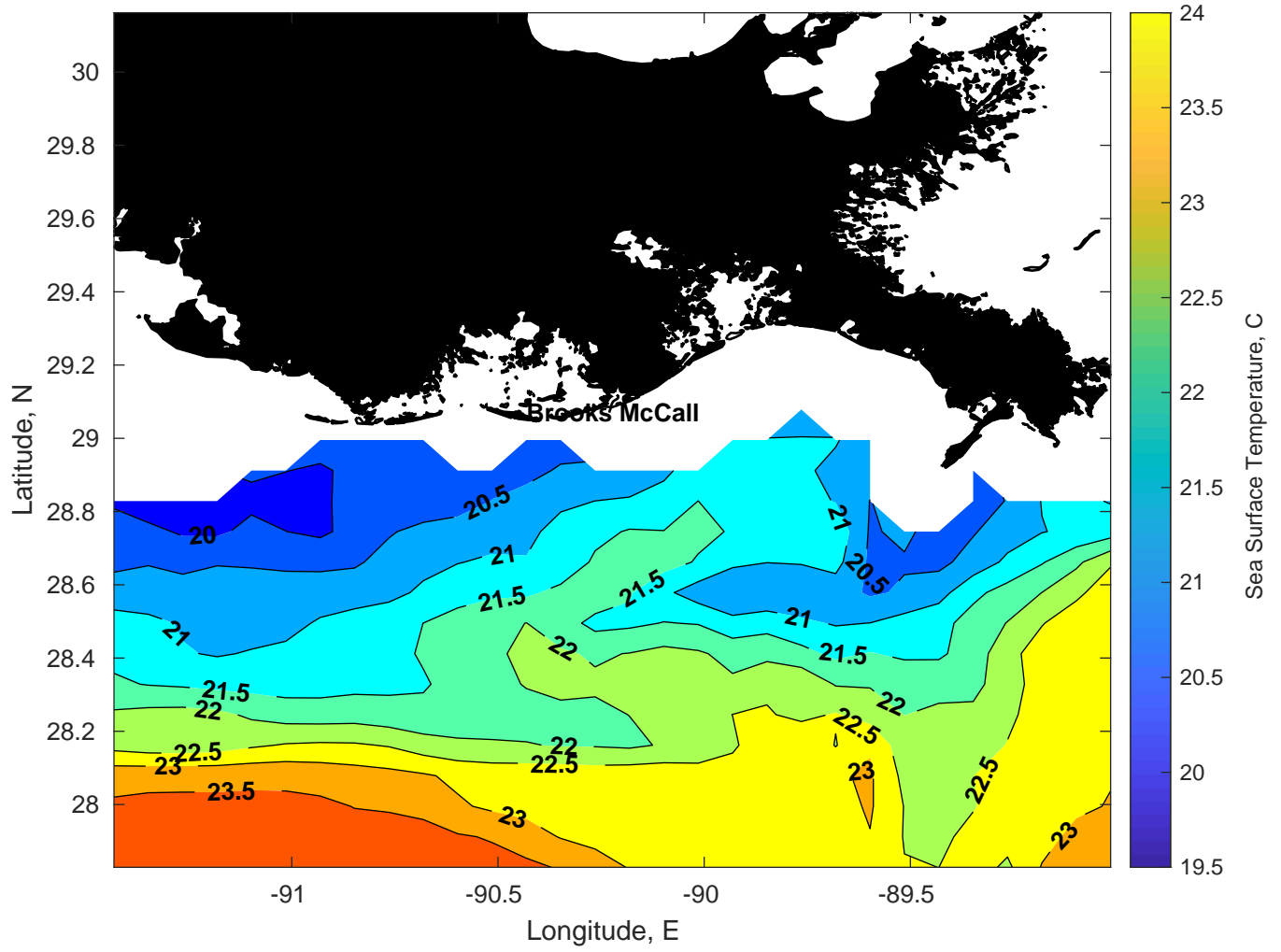
SST for Brooks McCall at 15-Mar-2025 00:00:00
