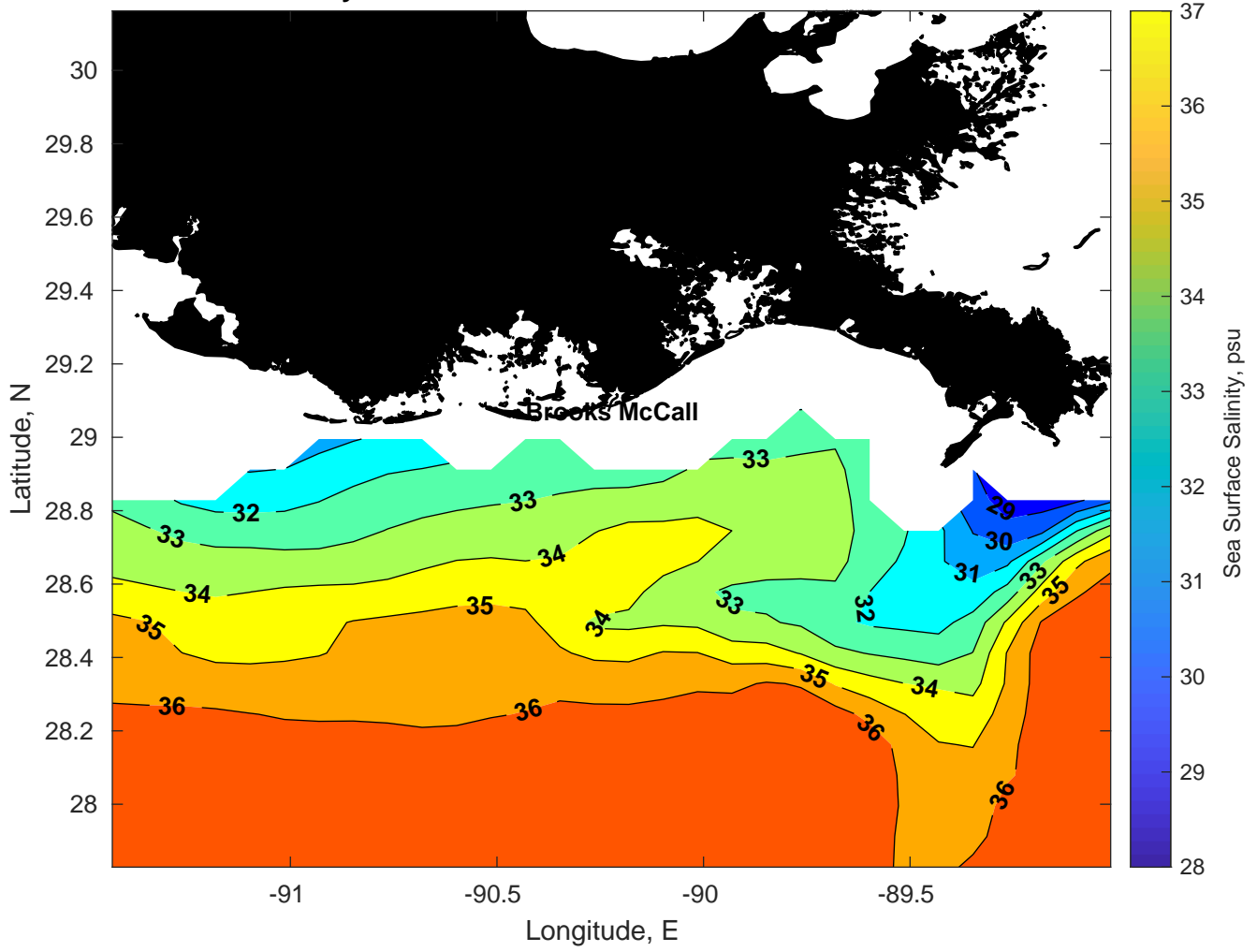
Surface Salinity for Brooks McCall at 15-Mar-2025 00:00:00
