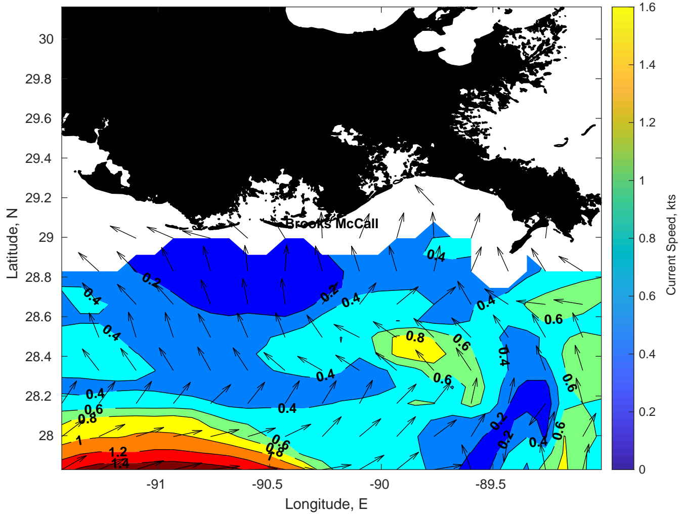
Surface Currents for Brooks McCall at 15-Mar-2025 00:00:00
