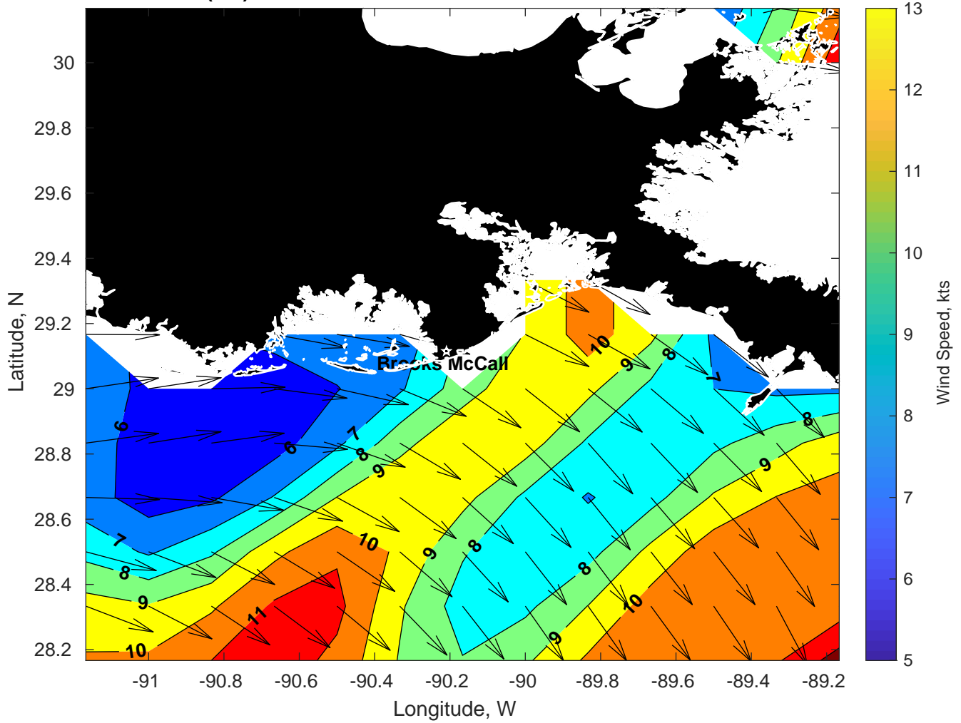
Winds (kts) for Brooks McCall at 16-Mar-2025 09:00:00
