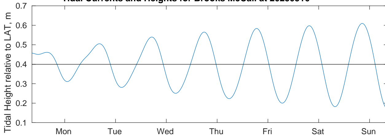
Tidal Currents and Heights for Brooks McCall at 20250316
