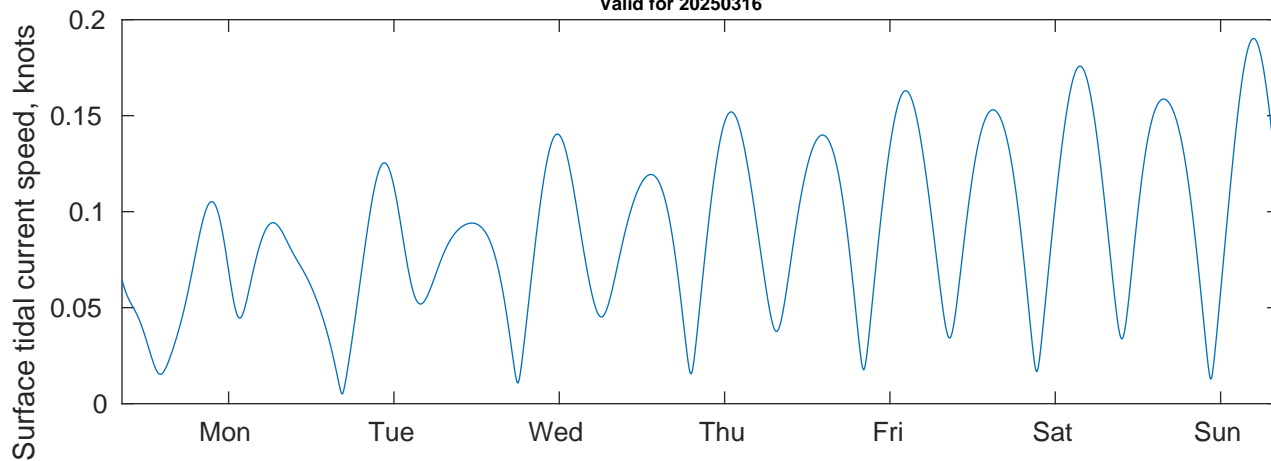
Tidal Currents and Heights for Brooks McCall at 20250316
