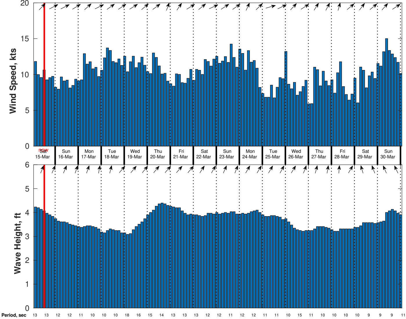
Wind & Wave Forecast for CSA (ONHYM) PPL EBS - Ghana from 14-Mar-2025 02:00:00 to 30-Mar-2025 02:00:00
