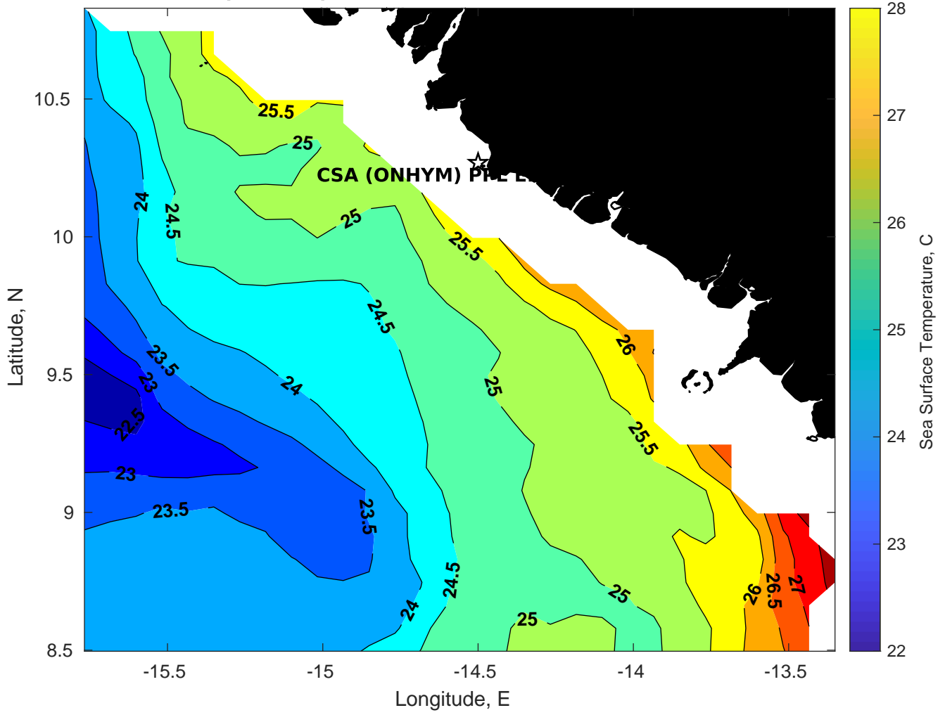
SST for CSA (ONHYM) PPL EBS - Guinea at 13-Mar-2025 00:00:00
