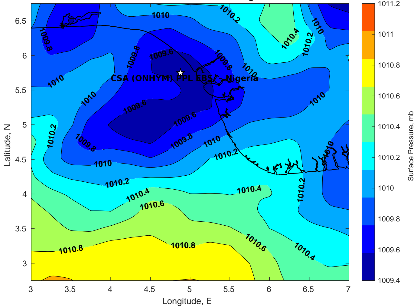
Surface Pressure (mb) for CSA (ONHYM) PPL EBS - Nigeria at 15-Mar-2025 00:00:00
