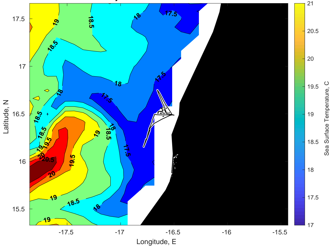
SST for Gyre at 15-Mar-2025 00:00:00
