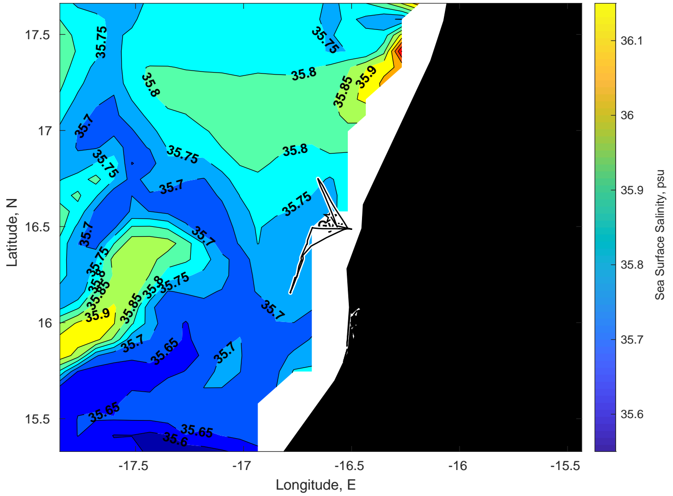
Surface Salinity for Gyre at 15-Mar-2025 00:00:00
