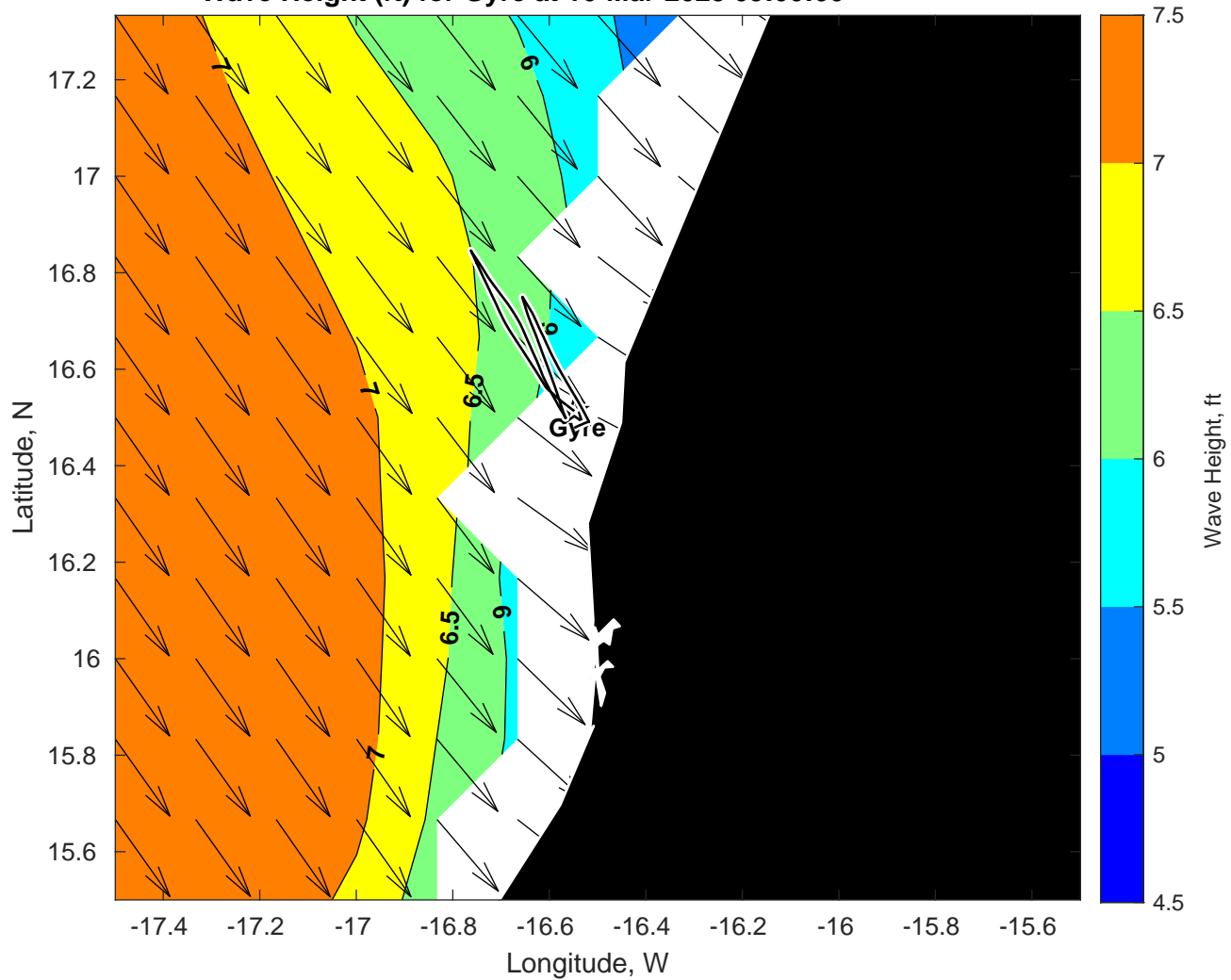
Wave Height (ft) for Gyre at 16-Mar-2025 09:00:00
