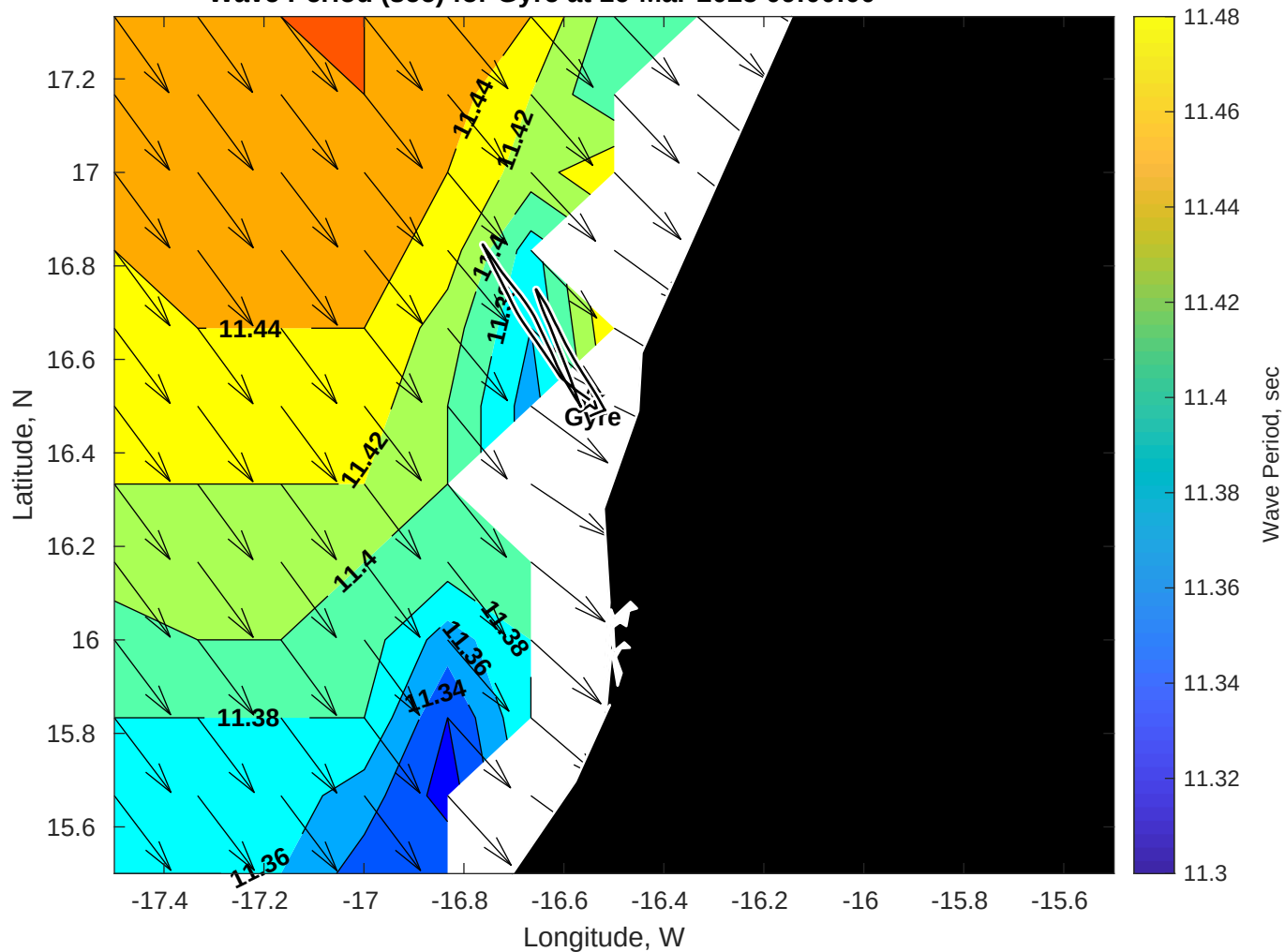
Wave Period (sec) for Gyre at 16-Mar-2025 09:00:00
