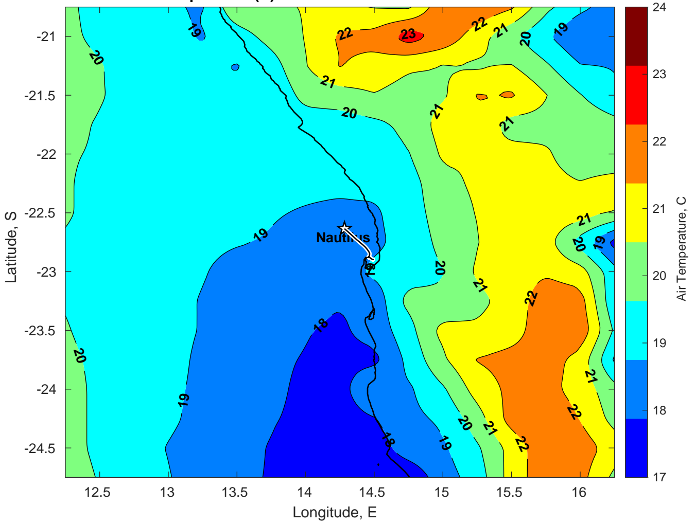
Air Temperature (C) for Nautilus at 14-Mar-2025
