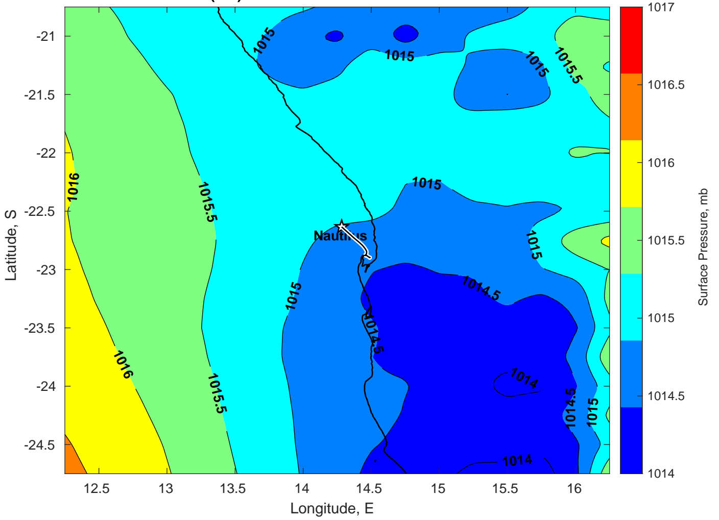
Surface Pressure (mb) for Nautilus at 16-Mar-2025 00:00:00
