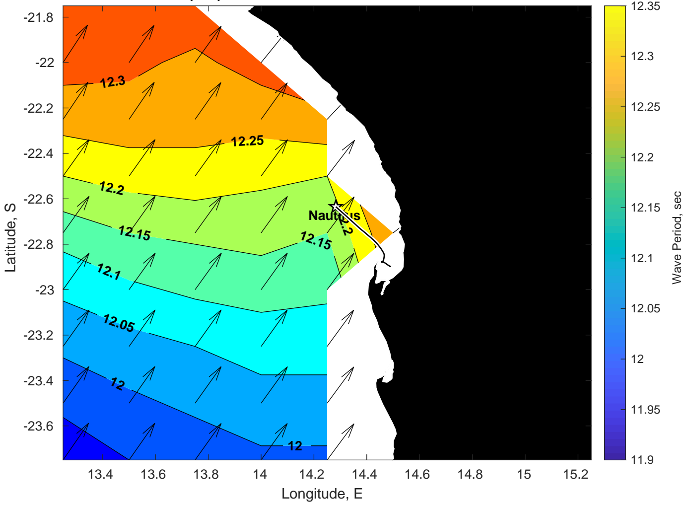
Wave Period (sec) for Nautilus at 14-Mar-2025 09:00:00
