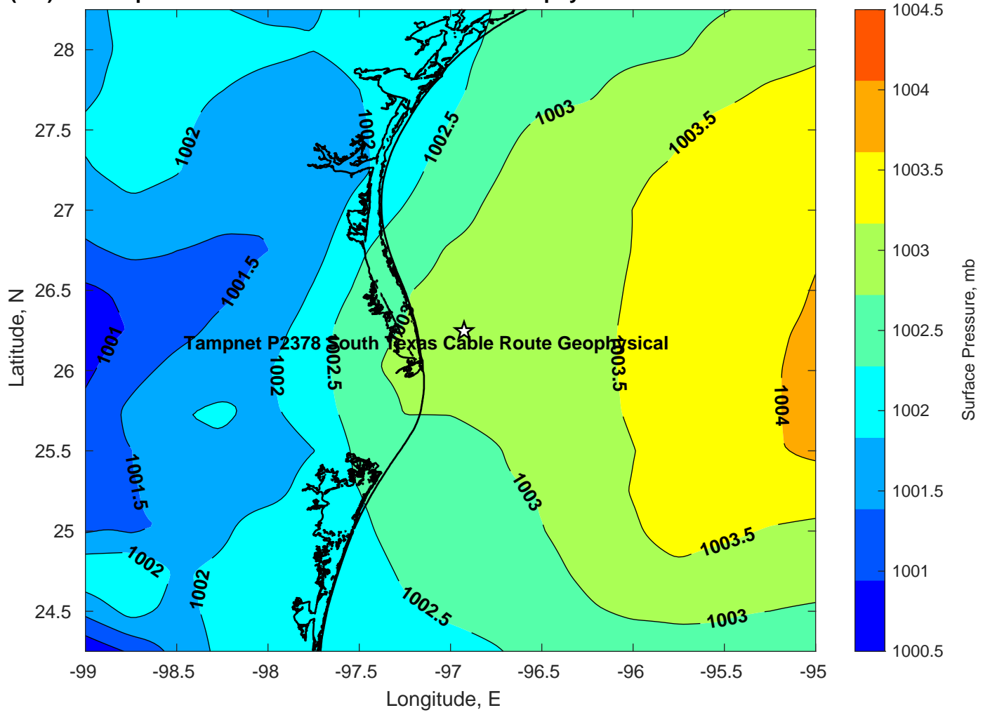
Pressure (mb) for Tampnet P2378 South Texas Cable Route Geophysical at 16-Mar-2025 00:00:00
