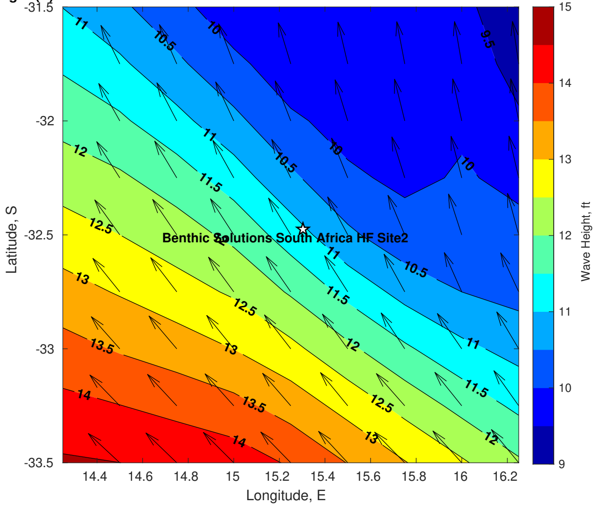
Wave Height (ft) for Benthic Solutions South Africa HF Site2 at 14-Mar-2025 09:00:00
