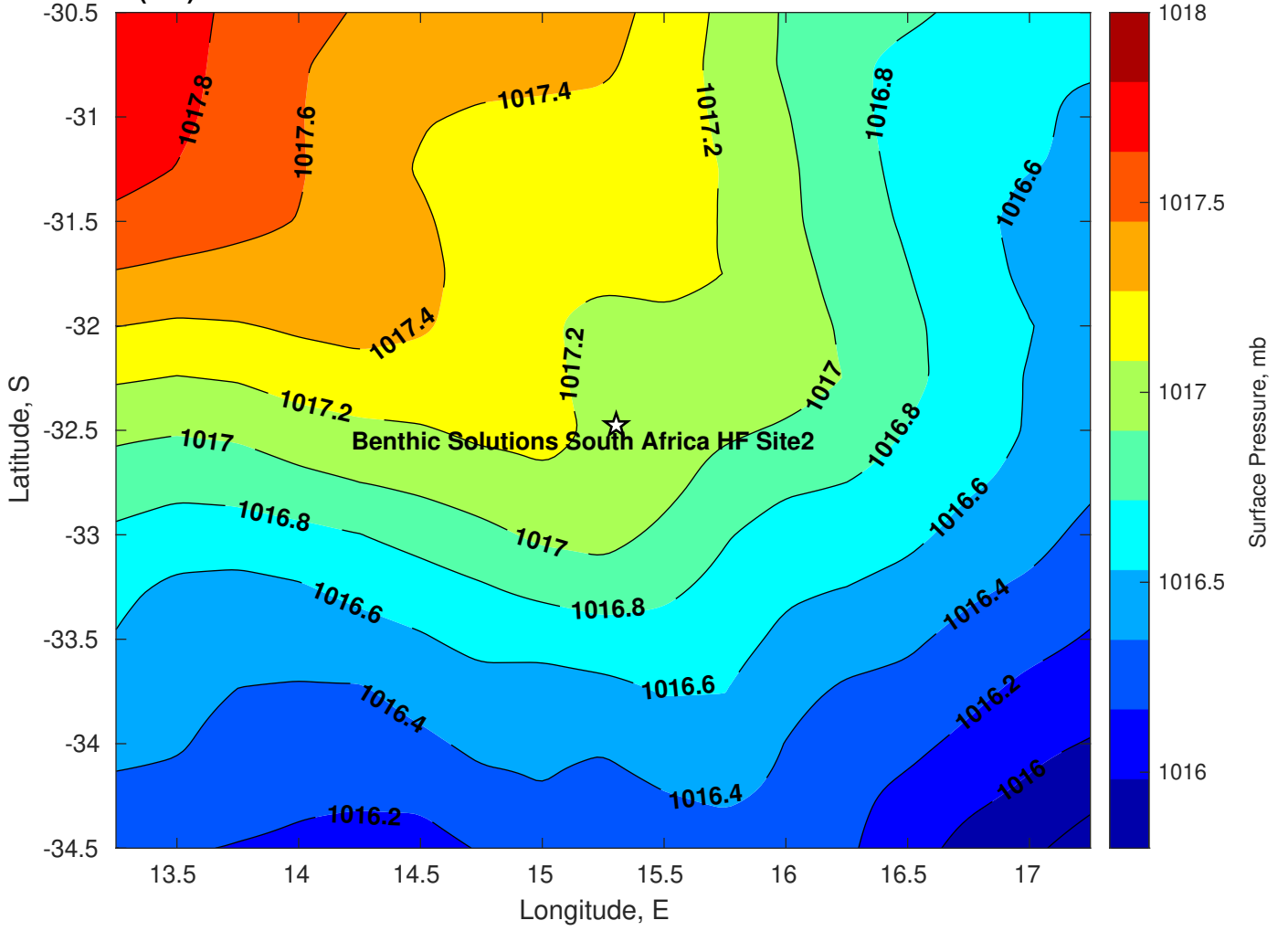
Surface Pressure (mb) for Benthic Solutions South Africa HF Site2 at 16-Mar-2025 00:00:00
