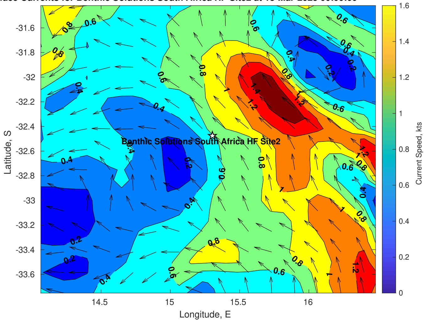
Surface Currents for Benthic Solutions South Africa HF Site2 at 13-Mar-2025 00:00:00
