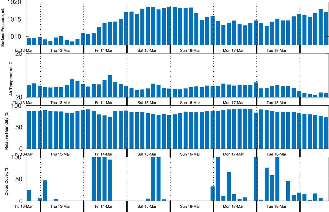
Met Forecast for Benthic Solutions South Africa HF Site2 from 13-Mar-2025 12:00:00 to 20-Mar-2025 12:00:00
