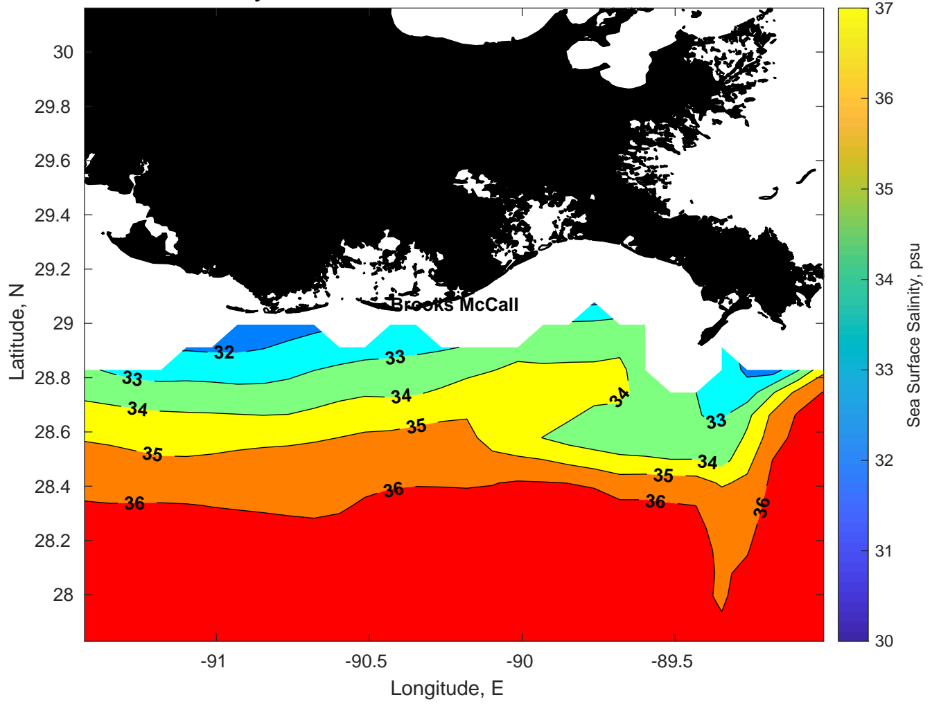
Surface Salinity for Brooks McCall at 16-Mar-2025 00:00:00
