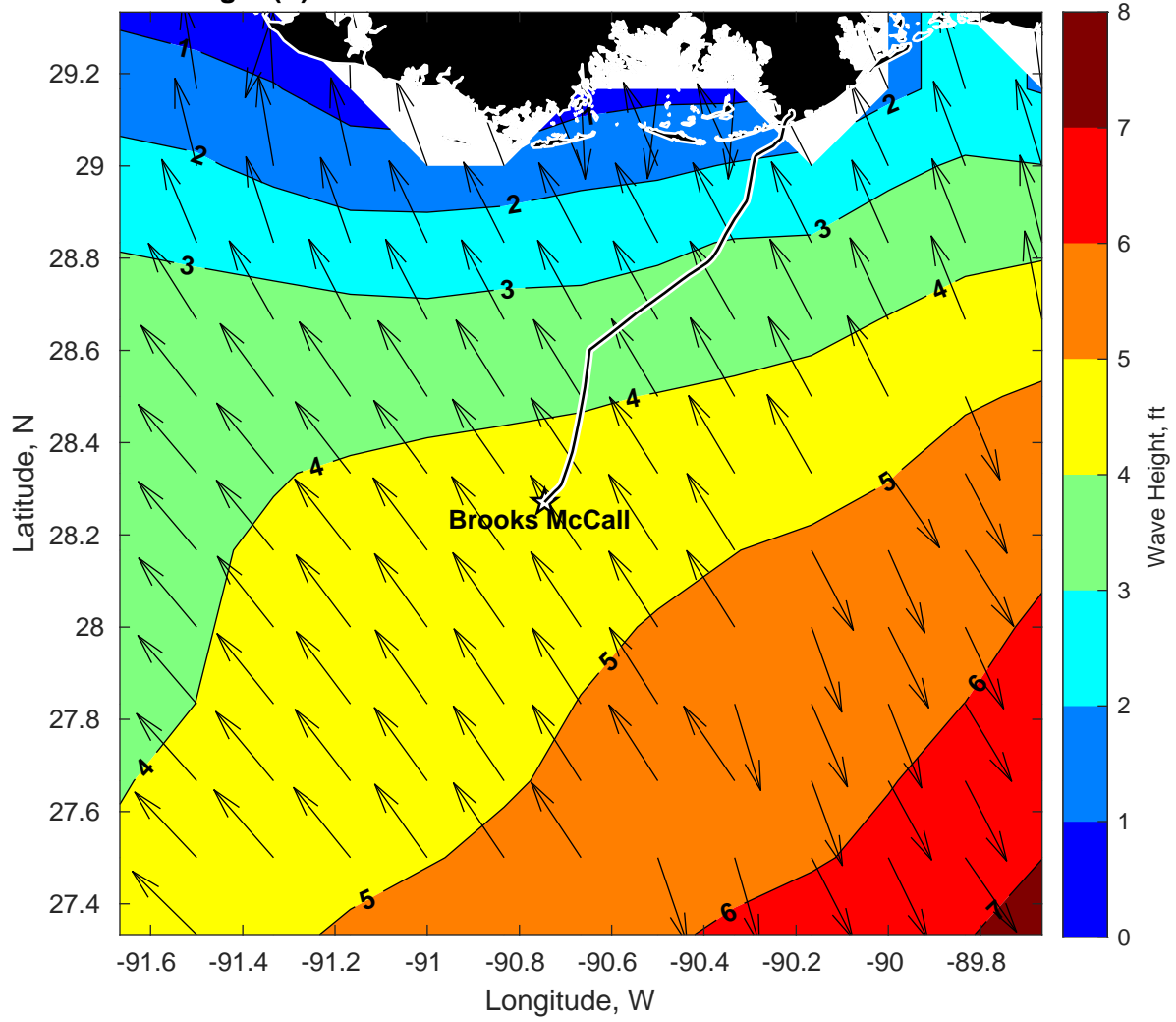
Wave Height (ft) for Brooks McCall at 17-Mar-2025 09:00:00
